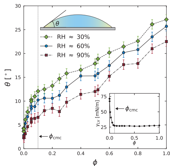
Figure 1. Contact angle ( \theta ) of water–1,2-HD mixtures as a function of the mass fraction ( \phi ) of 1,2-HD for various RH. The vertical dotted line indicates the cmc ( \phi_{\text{cmc}} \approx 0.1 ). Schematic: Definition of \theta . The mass fraction of 1,2-HD (yellow) is higher near the contact line due to selective evaporation. Inset: Surface tension ( \gamma_{LV} ) of water–1,2-HD mixtures, measured using the pendant drop method.
