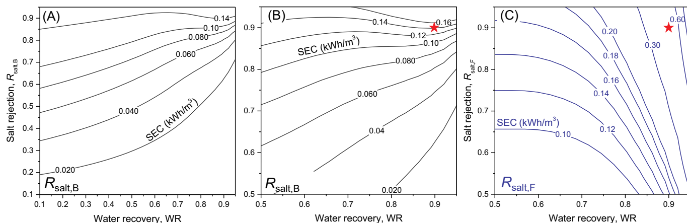
Fig. 1. (A) A reproduction of the calculated specific energy consumption from Qin et al. [1] for RO (their Fig. 8B) as function of water recovery (WR) and salt rejection calculated using brine water concentration ( R_{\text{salt,B}} ) (Eq. (1)). (B) The same plot as in Fig. 1A with WR > 50\% and R_{\text{salt}} > 50\% . (C) RO specific energy consumption as function of WR and the salt rejection calculated using feed water concentration ( R_{\text{salt,F}} ) (Eq. (2)). Feed salinity 2 g/L, and membrane flux 10 \text{ L m}^{-2} \text{ h}^{-1} . The red star indicates a desalination with WR = 0.9 and R_{\text{salt}} = 0.9 , and if R_{\text{salt}} is calculated based on the brine water concentration, SEC = \sim 0.14 \text{ kWh/m}^3 (Fig. 1B), and based on the feed water concentration SEC = \sim 0.45 \text{ kWh/m}^3 (Fig. 1C), which is a difference of around a factor of 3.5.
