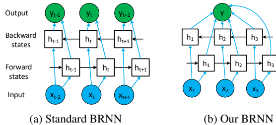
Figure 5: The standard BRNN model [33] (a), and (b) our BRNN model used for predicate prediction. Our BRNN has three inputs in sequence ( subject , spatial information and object ) and one output (predicate prediction).
