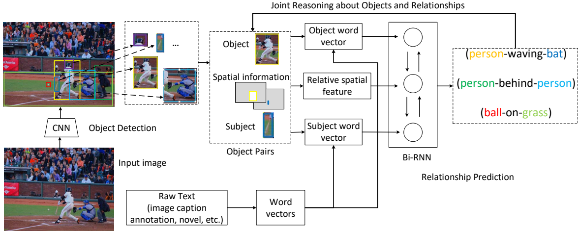
Figure 3: The proposed framework for visual relationship detection. First, Faster RCNN is utilized to localize objects and provide the classification probability of each detected object in the given image. Then, the possible meaningful object pairs are selected as the candidate relationships. Each object converted into the corresponding word vector.
