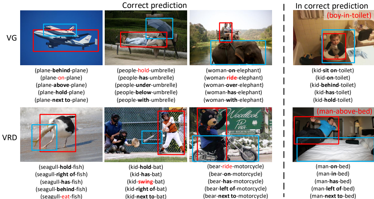
Figure 8: Qualitative examples of visual relationships detection on VG [17] (the first row) and VRD [24] (the second row) respectively. The first three columns illustrate the correctly recognized relationships in the images, while the last column is the failure example (the ground truth relationship phrase is denoted in red in the image). The red bounding boxes denote the subjects while the cyan boxes denote the objects. The relationships under the images are the Top - 5 most probable relationships predicted by our method, in which the red denotes the ground truth.
