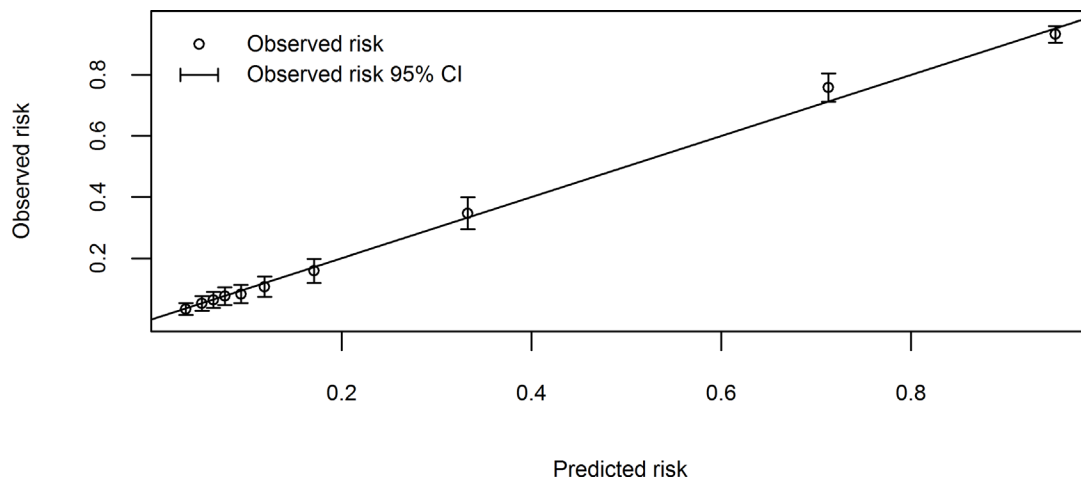
Fig 3. Calibration plot of the final 10-predictor model applied to the 3263 cases excluding subjects who were unconscious or who had experienced convulsions (Hosmer-Lemeshow goodness-of-fit p-value = 0.53). The 45 degree straight line corresponds to the line of perfect calibration on which model predicted risks coincide with the observed risks.
