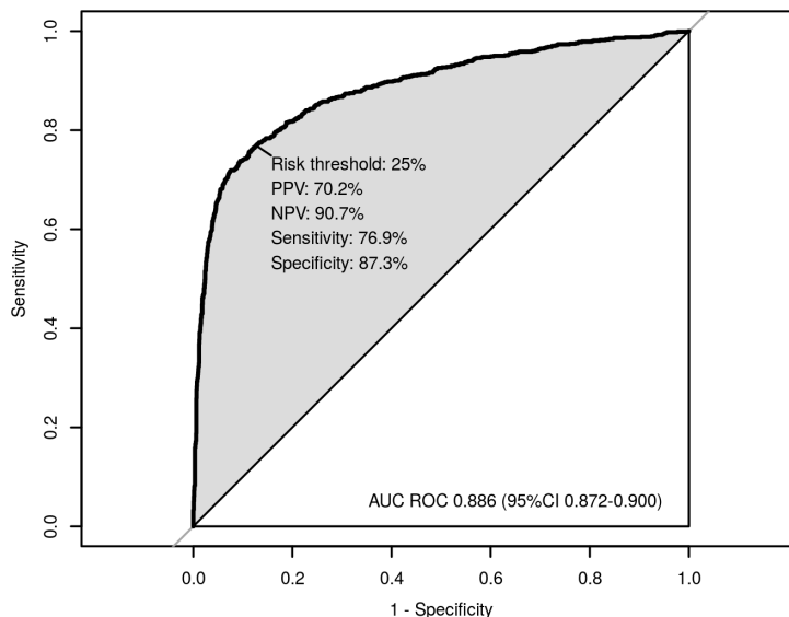
Fig 2. Receiver operating characteristic curve of the final model in the study cohort. AUC ROC = area under the curve of the receiver operating characteristic. Sens = sensitivity. Spec = specificity. PPV = positive predictive value. NPV = negative predictive value.
