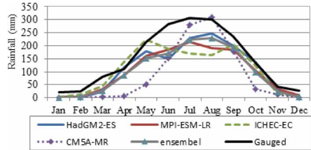
Figure 4 | Rainfall annual cycle over the Arjo-Didessa catchment from dynamically downscaled climate model simulations and gauged data on a monthly basis.
