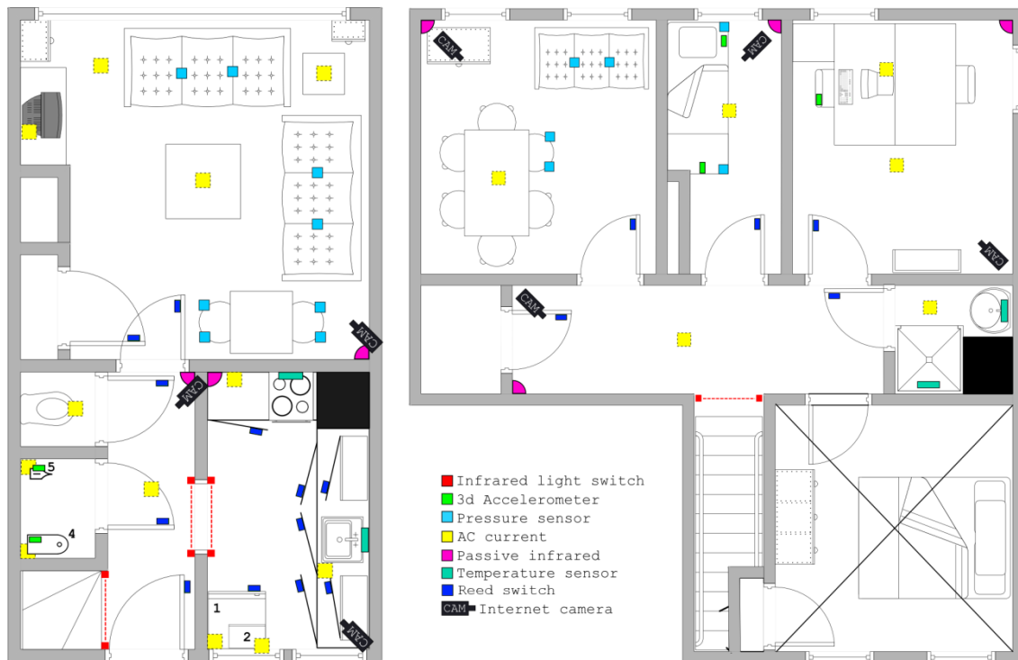
Figure 1: Floor plans of the ground floor (left) and upper floor (right) of the experiment house, including sensors and cameras.
