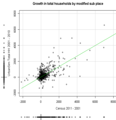
Figure 7 (a): Household growth between 2001 and 2011: Comparing UrbanSim predictions with Census 2011 data
