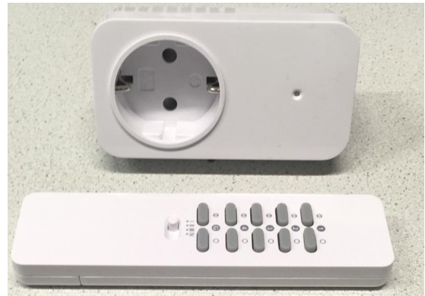
Fig. 1. COTS switch with dimming functionalities initially bought with the idea of using it as an on and off switch
