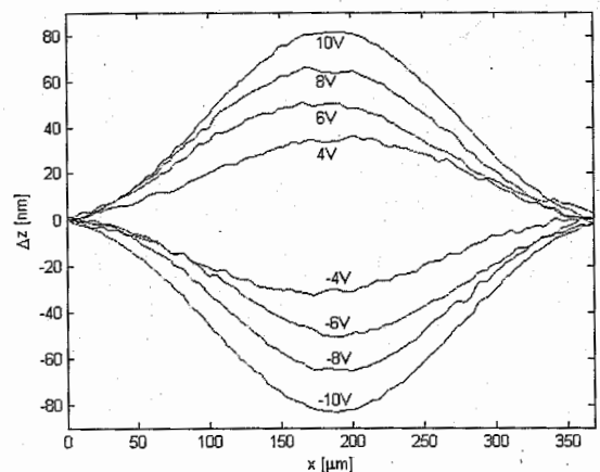
Fig. 6. Deflection profiles of a microbridge for various voltages from +10 V to -10 V.
