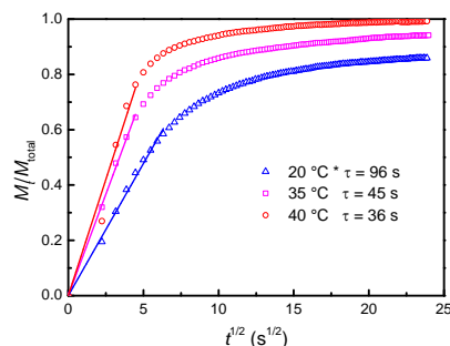
Fig. 6: Representative release curves (symbols) of IgG from 0.5 μm thick gelatin layers dried at different temperatures and fits of the initial release according to Eq. (1) (lines). The asterisk indicates “standard conditions”. Release times ( \tau ) are values for the specific release experiments shown here.
