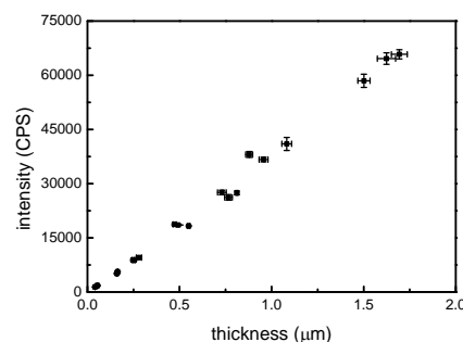
Fig. 3: Calibration of the fluorescence intensity of the layer against the layer thickness. Data points represent mean \pm standard deviation ( n=3 ).
