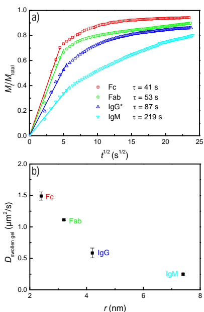
Fig. 8: (a) Representative release curves (symbols) of antibodies with different MWs from 0.5 \mu\text{m} thick layers and fits of their initial release according to Eq. (1) (lines). The asterisk indicates “standard conditions”. Release times ( \tau ) are values for the specific release experiments shown here. (b) Diffusivity ( D_{\text{swollen gel}} ) of antibodies and antibody fragments. Data points represent mean \pm standard deviation ( n=3 ).
