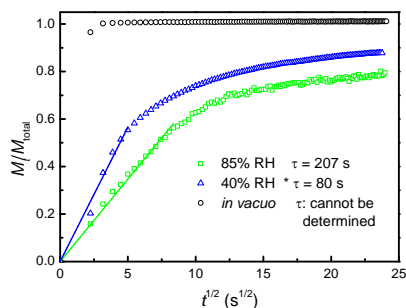
Fig. 7: Representative release curves (symbols) of IgG from 0.5 \mu\text{m} thick layers dried under reduced pressure (0.2 bar, black circles), ambient atmosphere (blue triangles) and 85% RH (green squares) and fits of the initial release according to Eq. (1) (lines). The asterisk indicates “standard conditions”. Release times ( \tau ) are values for the specific release experiments shown here.
