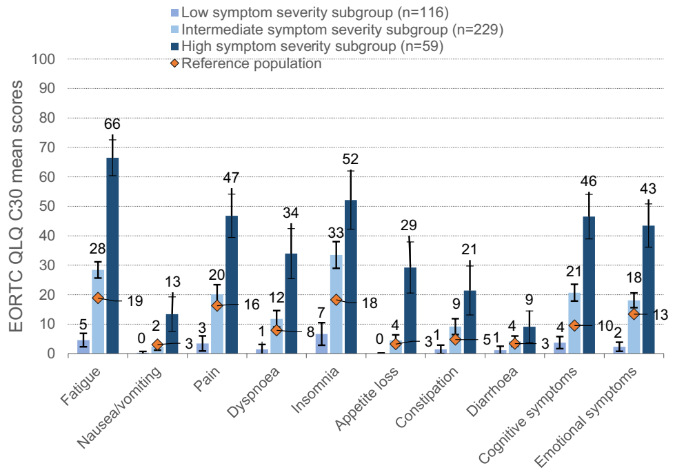
Fig. 1 Mean symptom severity per patient cluster versus reference population, including 95% confidence intervals. CI, confidence interval
