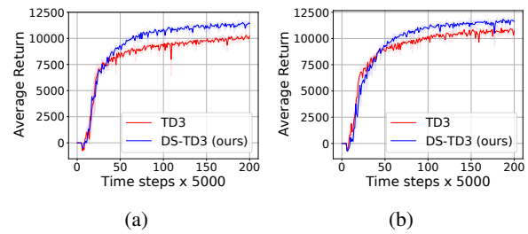
Figure 3: Learning curves of agents that start training with samples drawn from policies trained for 5 \times 10^5 (a) and 7 \times 10^5 steps (b).
