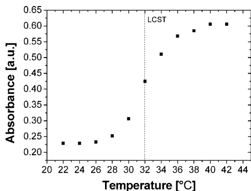
Figure 4. Absorbance ( \lambda_{\text{ex}} = 500 \text{ nm} ) of PNIPAM/QD microspheres as a function of temperature. The LCST temperature is determined to be 32 \text{ }^\circ\text{C} by plotting the first derivative of the data.
