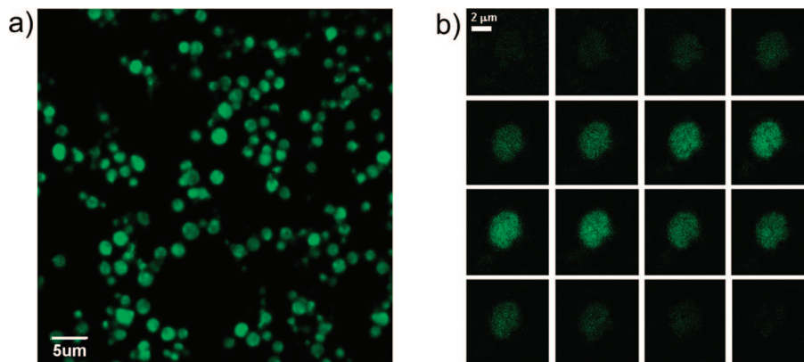
Figure 3. (a) A 50 \times 50 \mu\text{m}^2 scanning confocal fluorescence image of PNIPAM/QD spheres deposited on glass cover slides. (b) Scanning confocal cross-sectional z -scan of a single PNIPAM/QD microsphere. The QDs are uniformly distributed throughout the bead volume.
