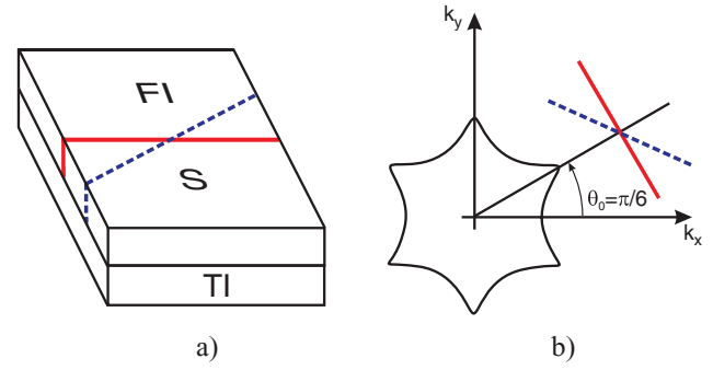
Figure 2. (a) Schematic illustration of the structure under consideration: superconductor/ ferromagnetic insulator (S/FI) junction formed on the surface of a three-dimensional topological insulator, TI. The x -axis is chosen perpendicular to the S/FI boundary. Two possible S/FI boundaries are shown by solid red and dashed blue lines as explained in figure (b). (b) Two possible alignments of the S/FI boundary with respect to the snowflake constant energy contour of the warped Dirac cone. The one, shown by solid red line, is favorable for the Majorana bound state realization, see details in the text. There are overall six favorable alignments at \theta_n values, corresponding to the six tips of the snowflake contour. The favorable alignment should be perpendicular to the line, connecting the tip and the center of the snowflake contour. Arbitrary boundary alignments, for example the one, shown by dashed blue line, are unfavorable and do not host the Majorana bound states.
