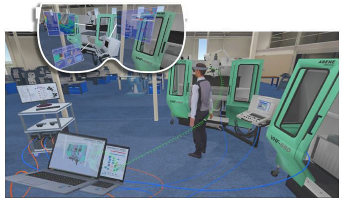
Fig. 5. Virtual Factory test setup at the University of Twente.
