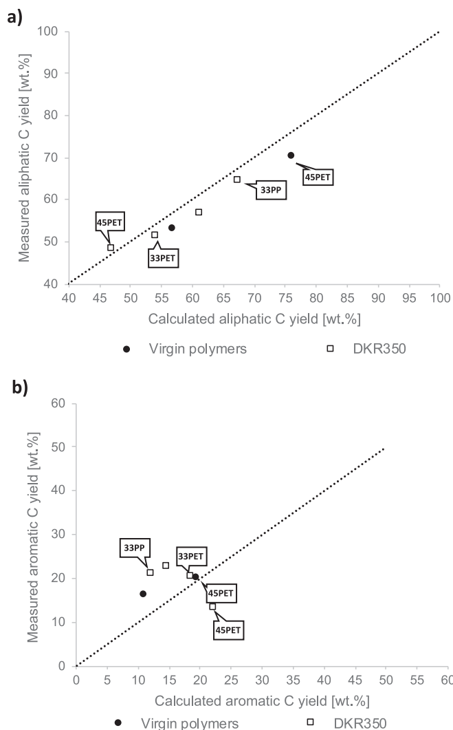
Fig. 7. Measured vs calculated yields of the aliphatic (a) and aromatic (b) carbon (wt.%) in the oil from pyrolysis of DKR-350 and mixtures of virgin polymers.
