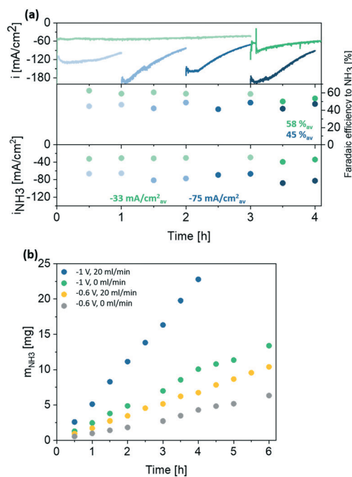
Fig. 6 (a) Stability test in 0.1 M \text{HClO}_4 with 50 mM \text{KNO}_3 at -1 V vs. RHE with 0 \text{ml min}^{-1} (green) and 20 \text{ml min}^{-1} (blue) flow rate showing overall current density as well as faradaic efficiency and partial current density to \text{NH}_3 . (b) \text{NH}_3 mass increase in stability test in different conditions.
