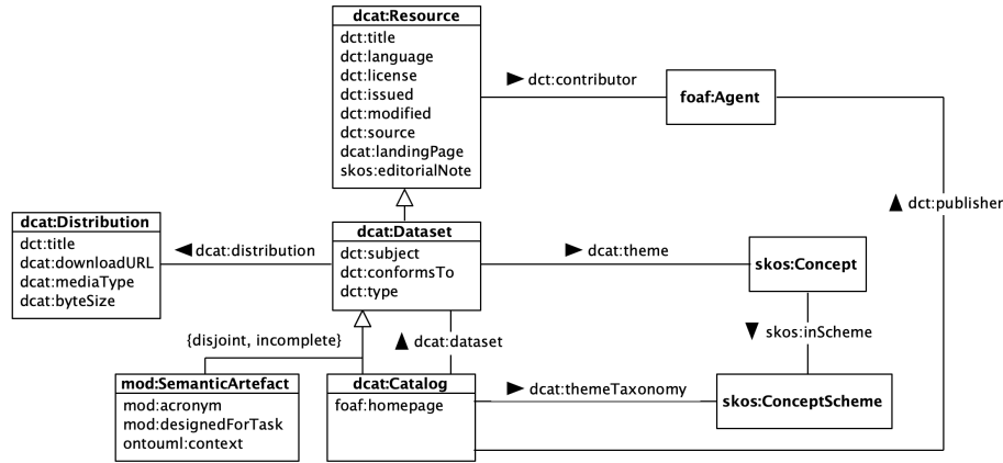
Fig. 1. The OntoUML/UFO Catalog schema in a UML class diagram representation.
