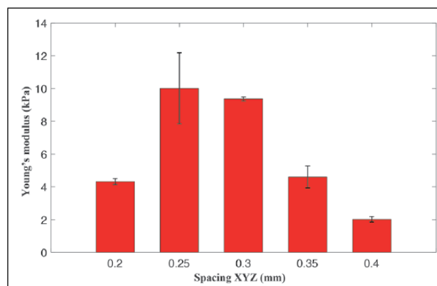
Figure 5. Young's moduli of a series of bioprinted cylindrical structures at different interline spacing, equally varied along the x , y , and z directions.
