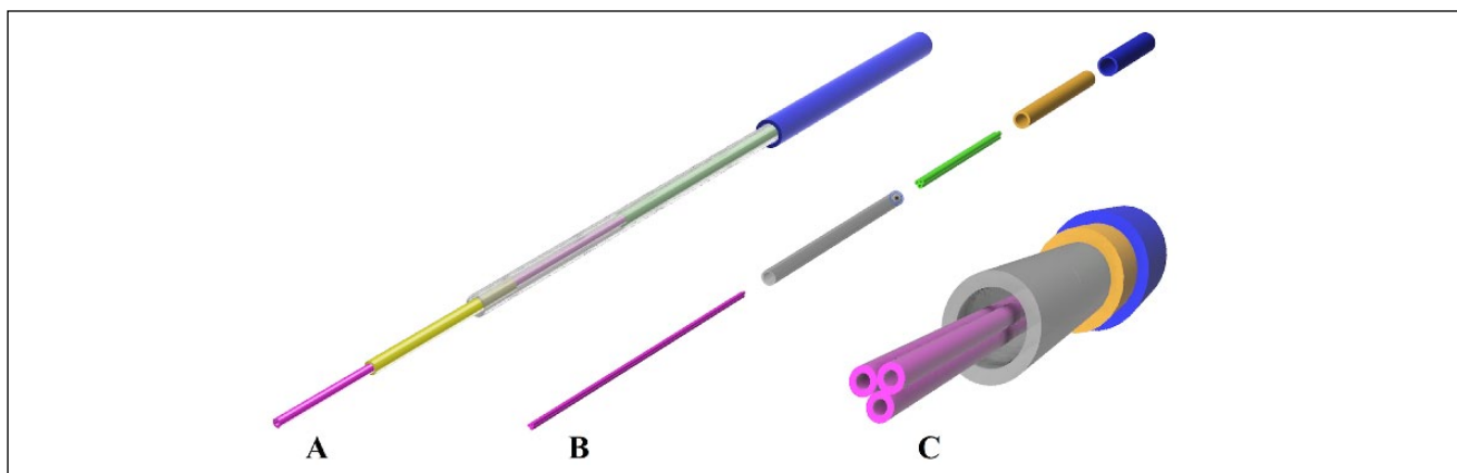
Figure 2. (A) Design of the single-nozzle printhead. A thin tip (30G) with an inner diameter of 159 \mu\text{m} was encased in increasingly larger metal tubes to maintain a small nozzle size at the tip while at the same time keeping a stiff and rigid overall structure. (B) Exploded view of the design of a multinozzle printhead. Three thin tips (30G) were fixed together to form the extrusion nozzle. This allowed for different materials to be extruded simultaneously or sequentially, while avoiding intermixing of the hydrogels prior to extrusion. Similar to the single-nozzle approach, a sequence of three metal tubes with increasing diameters were used to make the structure stiffer and avoid its bending. (C) Front view of the multinozzle printhead.
