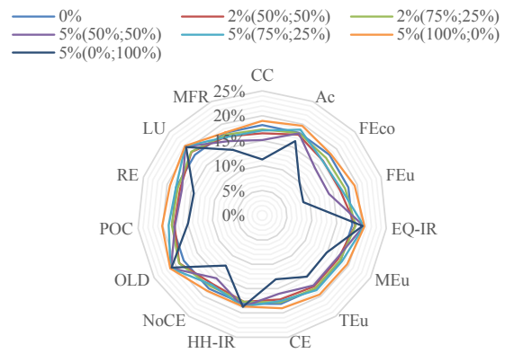
Fig. 3. Relative variation of the LCIA results obtained in the AS1 in relation to those corresponding to the use of conventional asphalt surface mixture (no PMB) in the baseline scenario. Key: Polymer%(NBR%;EVA%).
