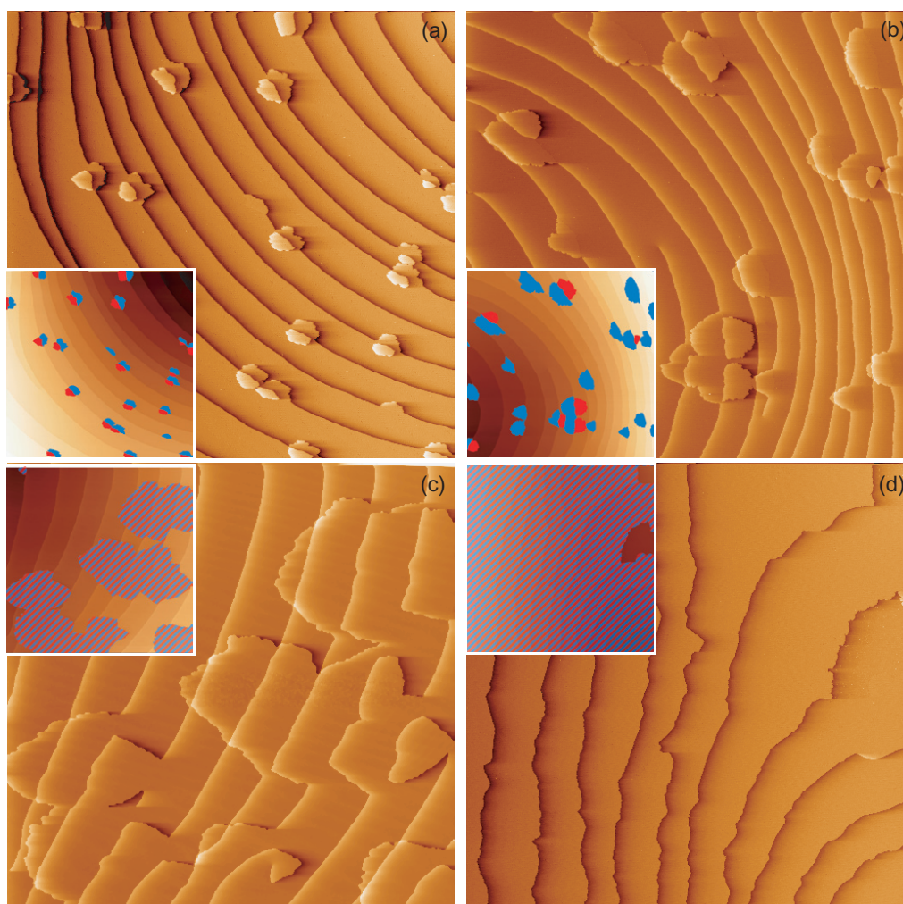
Figure 6. Differentiated STM topographs ( 1\ \mu\text{m} \times 1\ \mu\text{m} ) at 300 K of graphene grown on a Ir(111) surface at 1120 K, by exposure to an ethene partial pressure of 5 \times 10^{-10} mbar, during 20 s (a), 40 s (b), 160 s (c) and 320 s (d). Insets are scaled down versions of the large topographs: (a, b) graphene on lower (upper) terraces is marked blue (red) and (c, d) graphene areas are colored blue/red.
