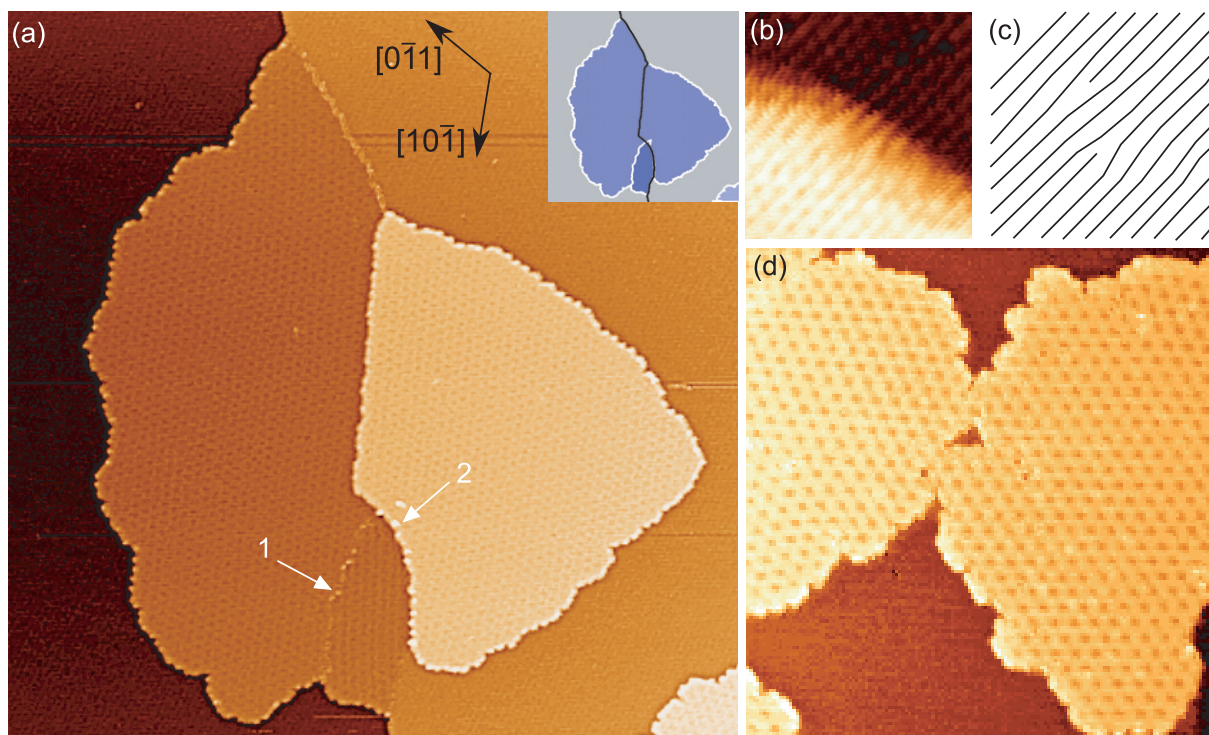
Figure 8. (a) STM topograph ( 171 \text{ nm} \times 171 \text{ nm} ) of graphene grown by CVD on a Ir(111) surface at 1120 K, out of exposure to an ethene partial pressure of 5 \times 10^{-10} \text{ mbar} , during 40 s. The arrows point out edge dislocations at the boundary between two moiré domains, at a terrace (1) and in close vicinity of the step edge (2). The black arrows show the orientation of the Ir(111) substrate throughout this figure. The inset shows the Ir(111) surface (gray) supporting graphene and exhibiting a step edge (black line). Different orientations of the moiré are visualized with blue tones. (b) STM topograph ( 2.7 \text{ nm} \times 2.7 \text{ nm} ) of graphene across a substrate step edge, and (c) a corresponding line network of C rows showing two edge dislocations. (d) STM topograph ( 70 \text{ nm} \times 73 \text{ nm} ) of two coalesced islands forming a coherent graphene island (exposure to 5 \times 10^{-10} \text{ mbar} ethene for 20 s).
