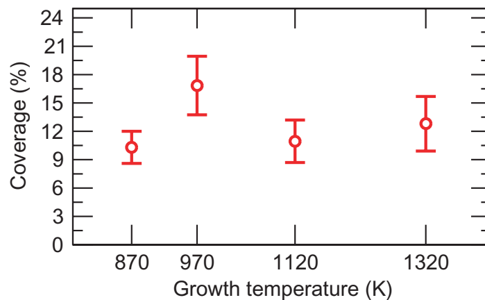
Figure 11. Graphene coverage as a function of the CVD growth temperature, for an ethene dose of 2 \times 10^{-8} mbar s.
