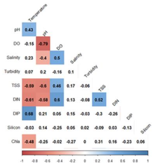
Figure 6. Correlation Matrix of Water Quality Parameters as Explanatory Variables with Significance Level (α) 0.05
