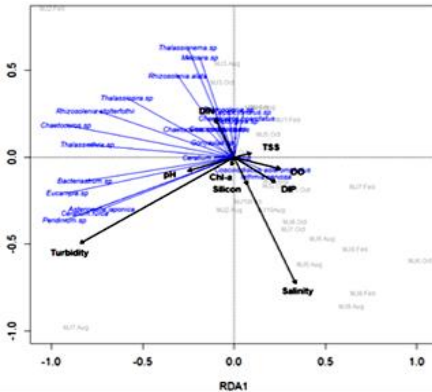
Figure 7. Result of RDA Shown as Canonical Ordination Triplot of RDA1 and RDA2 Axes, with the Elements of PHYTOPLANKTON Species, Samples and Water Quality Parameters Respectively Represented as Blue Lines, Grey Texts, and Black Arrows. Length of Arrows and Lines Represent the Relative Importance of the Variable or Species. The Distance between Samples Correlates the Dissimilarity in Species Composition, i.e., Close Samples in the Plot are more Similar than Distant Samples
