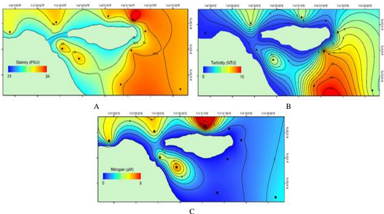
Figure 8. Spatial Visualization during CoTS Outbreak of Water Quality Variables with the Highest RDA score: (A) Salinity, (B) Turbidity, and (C) DIN
