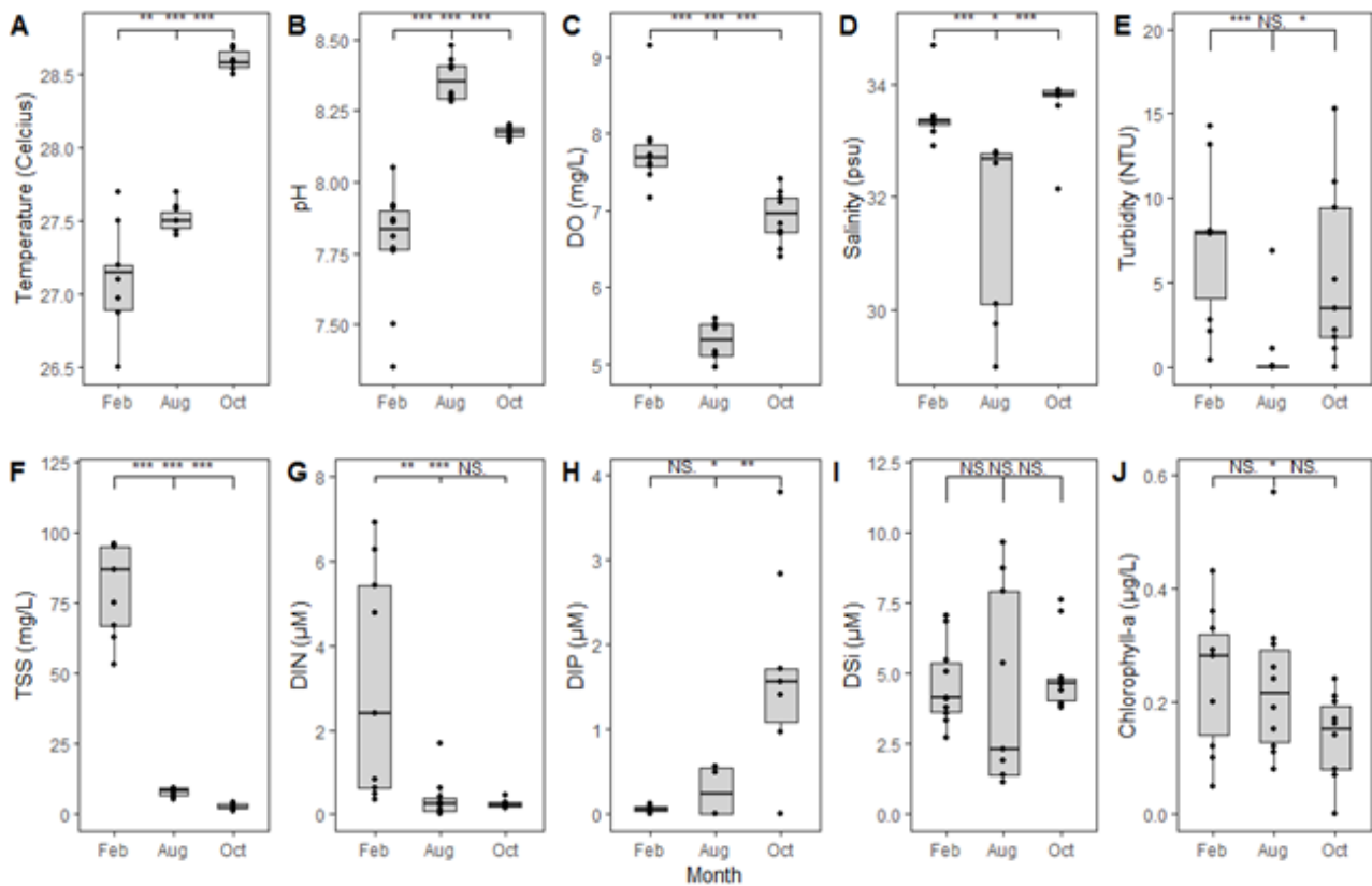
Figure 4. Box and Whisker Plot of Water Quality Parameters of 10 Sampling Stations in February, August, and October 2017. Note: Significance Test with p-value = 0.001 (***), 0.01 (**), 0.05 (*), and not Significant (NS). DO = Dissolved Oxygen, TSS = Total Dissolved Solids, DIN = Dissolved Inorganic Nitrogen, DIP = Dissolved Inorganic Phosphate, DSI = Dissolved Silicate
