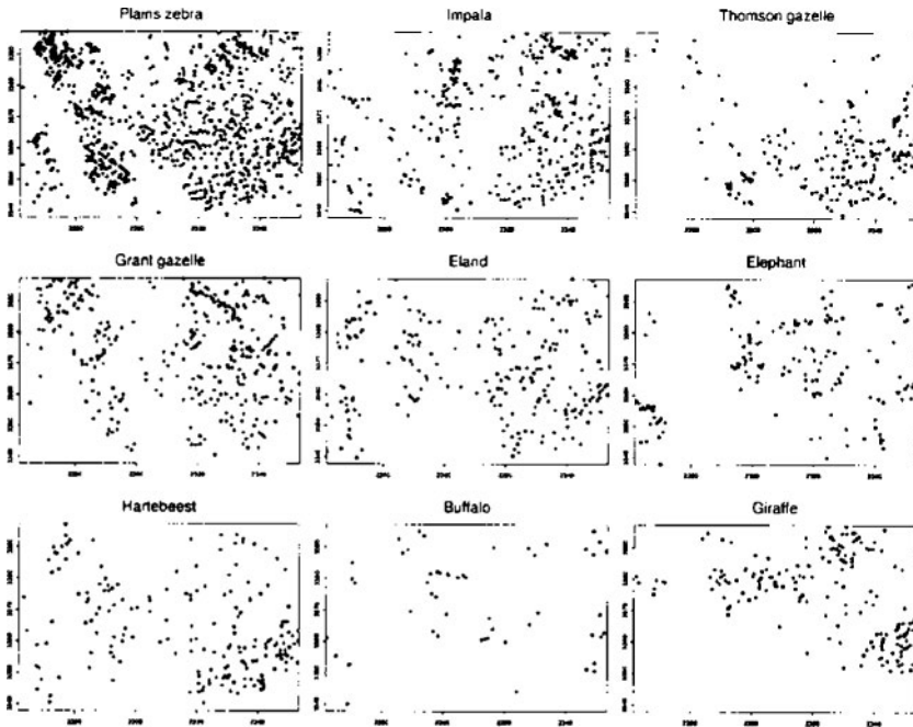
Figure 3.6. Spatial point patterns for the nine animal species in the study area. Coordinates are in km along a 55^\circ rotated image
