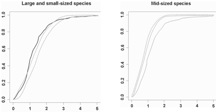
Figure 3.10. The estimated \hat{G}(r) function for large- and small-sized species (left-hand side) and mid-sized species (right-hand side). Coordinates along the horizontal axis are in km
