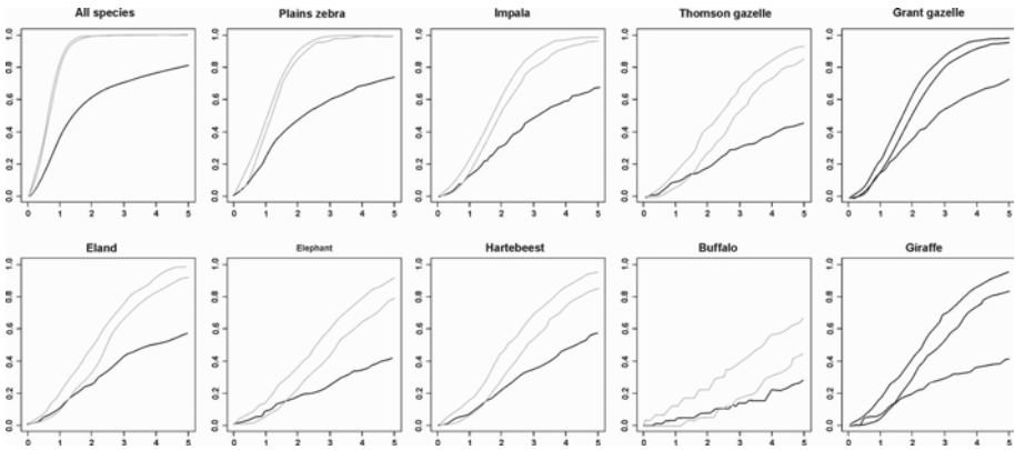
Figure 3.7. The estimated \hat{F}_\bullet(r) function for X_\bullet , the combined data, and the \hat{F}_i(r) -functions (solid lines) of the nine animal species with envelopes (dotted lines) for testing for spatial randomness. Coordinates along the horizontal axis are in km. The figure seems to imply regularity, as the estimated \hat{F}(r) functions are below the confidence bounds, both for all species and for each individual species. This is hard to justify, as a probable cause may be the empty sub-area in the northern part of the study area
