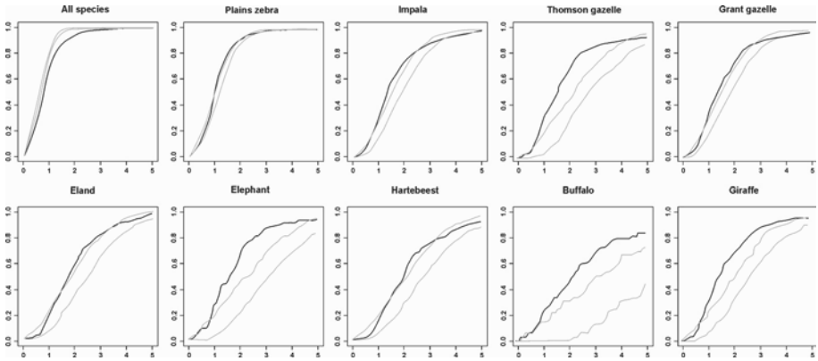
Figure 3.8. The estimated \hat{G}_\bullet(r) -function for X_\bullet , the combined data, and the \hat{G}_i(r) -functions (solid lines) for the nine animal species with envelopes (dotted lines) for testing for spatial randomness. Coordinates along the horizontal axis are in km. Figure numbering is from a (top left) to j (bottom right). All species show an aggregated pattern, with the exception of the plains zebra, which displays a random distribution. The pattern of all species, on the contrary, is more regularly distributed
