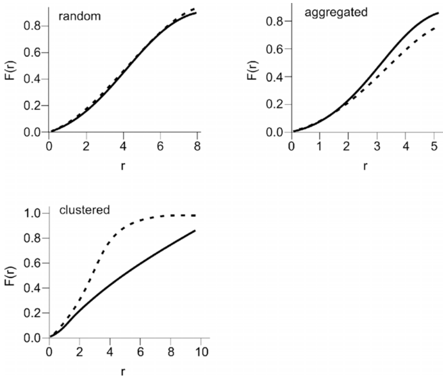
Figure 3.3. F-Functions for the random, aggregated and clustered processes. See Figure 3.2 for the corresponding patterns
