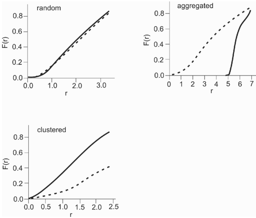
Figure 3.4. G -functions for the random, aggregated and clustered processes. See Figure 3.2 for the corresponding patterns
