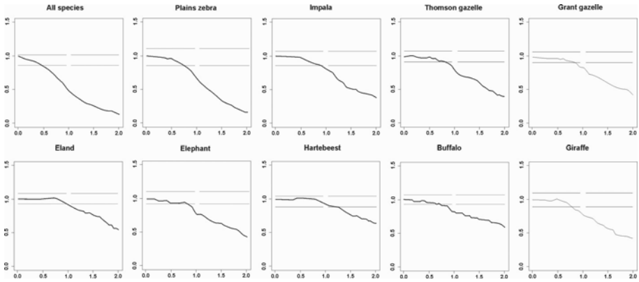
Figure 3.9. The estimated \hat{J}_\bullet(r) -function for X_\bullet , the combined data and the \hat{J}_i(r) -functions (solid lines) for the 9 animal species with envelopes (dotted lines) for testing for spatial randomness. Coordinates along the horizontal axis are in km. Figure numbering is from a (top left) to j (bottom right). These J -functions indicate randomness for distances up to 0.4 km (for all species) and to distances between 0.7 km and 1 km for individual species. Beyond that distance, herds are distributed in a more aggregated way
