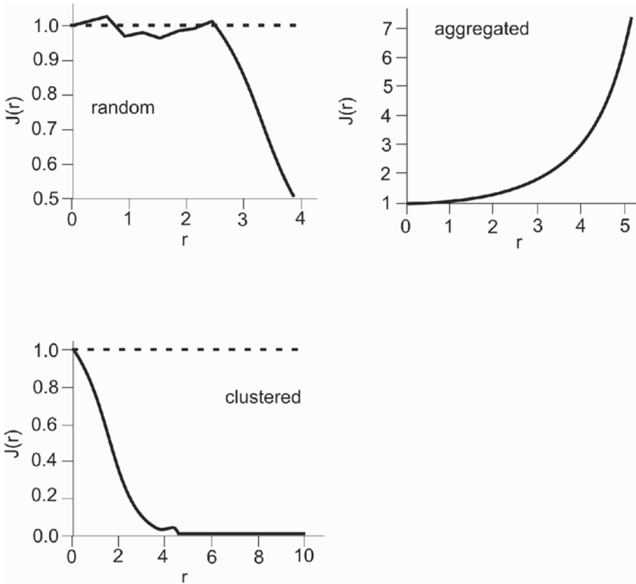
Figure 3.5. J -functions for the random, aggregated and clustered processes. See Figure 3.2 for the corresponding patterns
