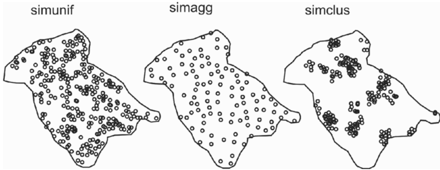
Figure 3.2. Simulated random ( simunif ), aggregated ( simagg ) and clustered ( simclus ) process in the Laikipia area. The patterns have 300, 100 and 191 herds, respectively. See Box 3.1 for further explanation
