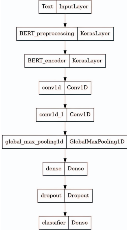
Fig. 1. Used BERT-CNN model architecture
