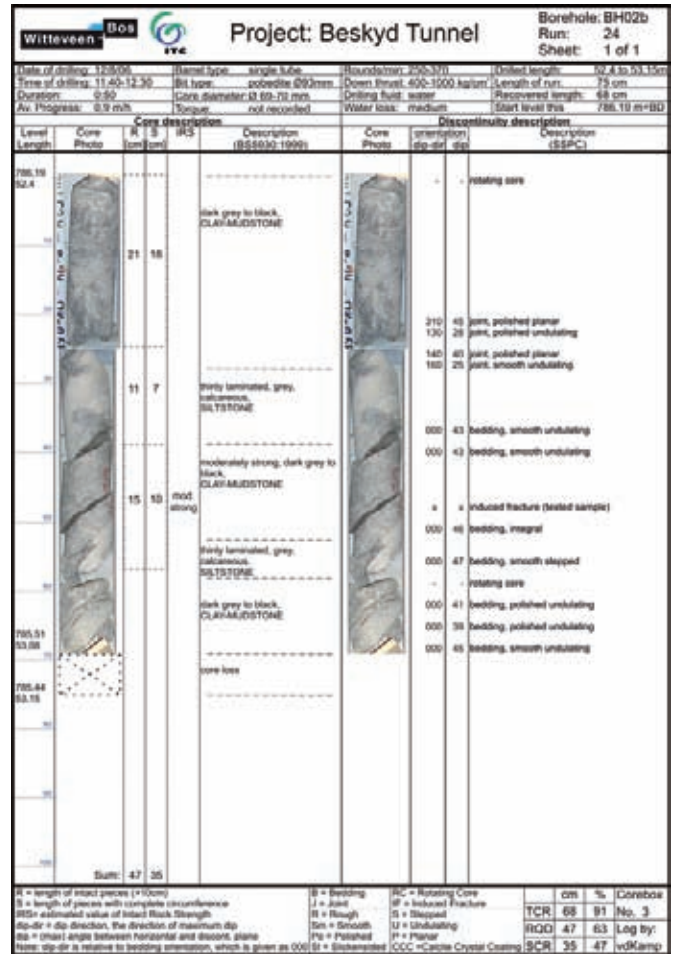
Figure 3. Example of borehole log
