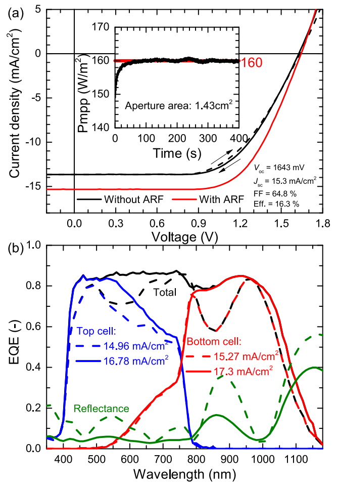
FIG. 4. (a) J - V measurements of the best performing >1 cm 2 monolithic tandem with and without antireflective foil (ARF). The inset shows the steady power output measured under maximum power point tracking; (b) EQE and total reflectance measurements of the same device as in (a), with (solid lines) and without (dashed lines) ARF. The total curve is the sum of the top and bottom cell responses.
