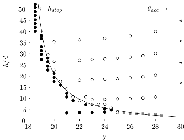
Fig. 2: Overview of DPM simulations for \mu^b = 0.5 , with markers denoting the state: arrested filled-symbols, steady open-symbols, and accelerating *. The demarcation line is fitted to h_{stop} in eq. (2) (solid line). Note, circular symbols are for increasing the number of particles and square symbols for decreasing.
