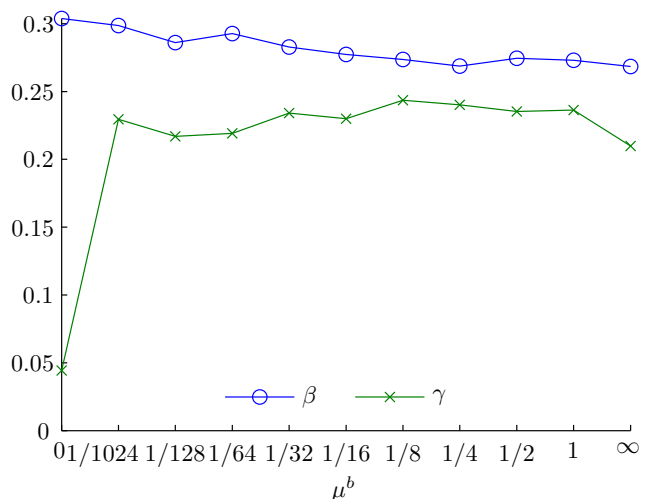
Fig. 5: Figure showing the dependence of \beta and \gamma on the contact friction coefficient between base and flowing particles \mu^b .
