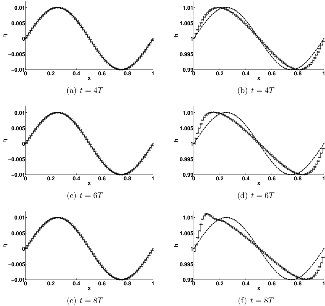
Figure 5: Numerical solution of harmonic waves using Port-Hamiltonian numerical scheme for linear (left) and nonlinear (right) shallow water equations on a grid of 80 elements. Exact and numerical solutions are marked as “* - *” and “o - o”, respectively. Observe in the left, numerical harmonic waves are in good agreement with the exact solution and in the right side, wave steepens due to nonlinearity.
