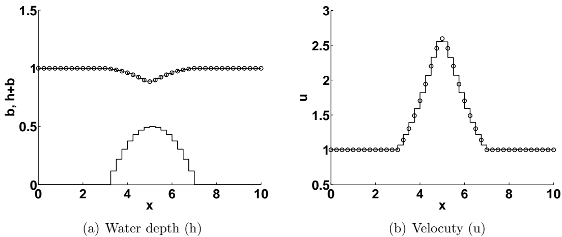
Figure 3: Comparison of numerical solution (“—”) of steady subcritical flow over bump against steady exact solution (“o”) on a mesh stencil with 40 elements.
