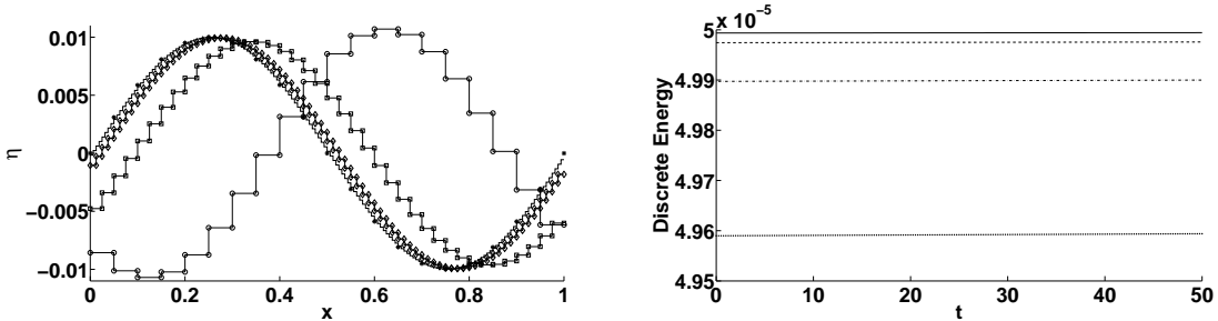
Figure 4: Left: Comparison of exact and numerical solution of free surface perturbation \eta(t, x) at time t = 50T . Exact solution is marked with “*” and numerical solution for 20 elements marked as “ \circ - \circ ”, 40 elements as “ \square - \square ”, 80 elements as “ \diamond - \diamond ” and 160 elements as “ \cdot - \cdot ”. Right: Total discrete energy in the computational domain with a grid of 20 “ \cdot - \cdot ”, 40 “ \square - \square ”, 80 “ \diamond - \diamond ” and 160 “ \circ - \circ ” elements.
