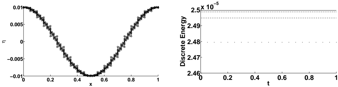
Figure 6: Left: Comparison of exact and numerical solution of free surface perturbation \eta(t, x) at time t = T . Exact solution is marked with “*” and numerical solution for 20 elements marked as “ \circ - \circ ”, 40 elements as “ \square - \square ”, 80 elements as “ \diamond - \diamond ” and 160 elements as “-”. Right: Total discrete energy in the computational domain with a grid of 20 “..”, 40 “-.-”, 80 “- -” and 160 “-” elements.
