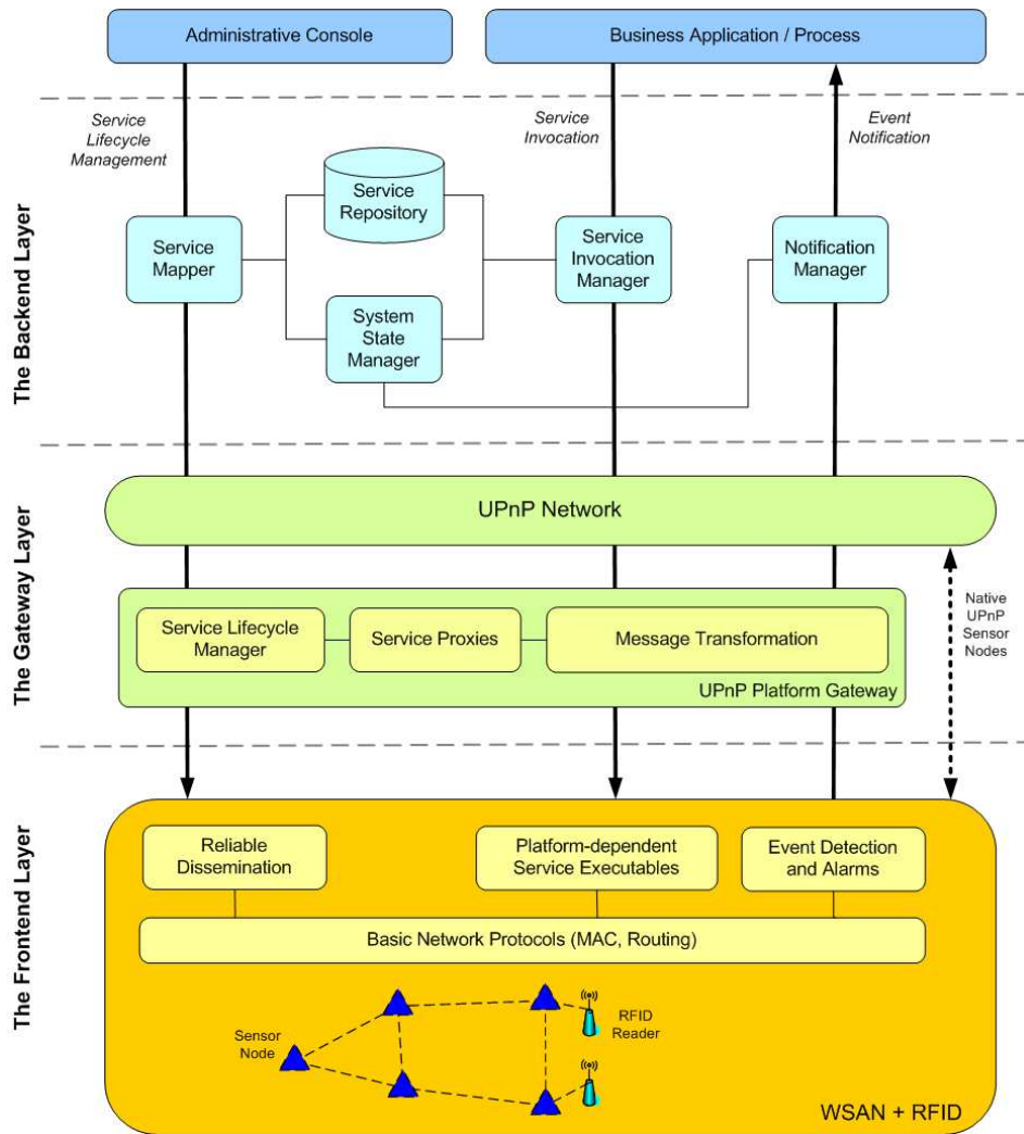
Fig. 3. Three-layer service-oriented architecture.
