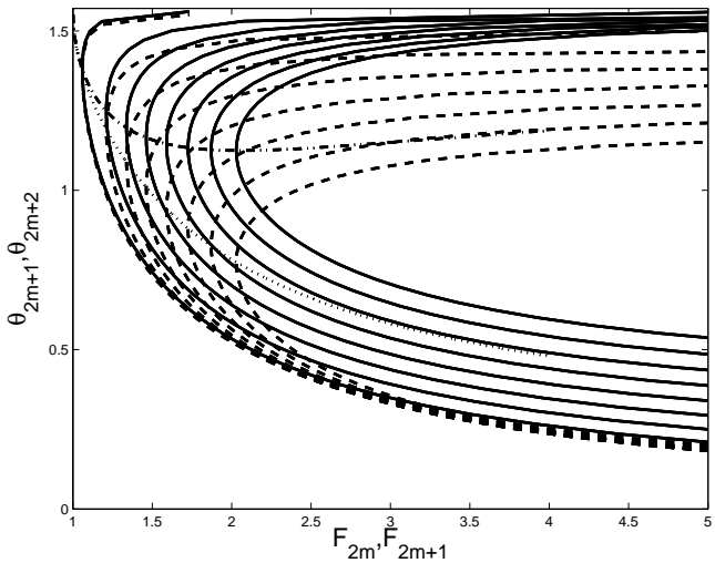
FIG. 10: Given various fixed angles \theta_c = 0, 0.05, \dots, 0.35 (going from left to right) of the contraction walls, the odd \theta_{2m+1} and even \theta_{2m+2} angles of the associated oblique jumps have been calculated as function of Froude numbers F_{2m} (solid lines) and F_{2m+1} (dashed lines), respectively.
