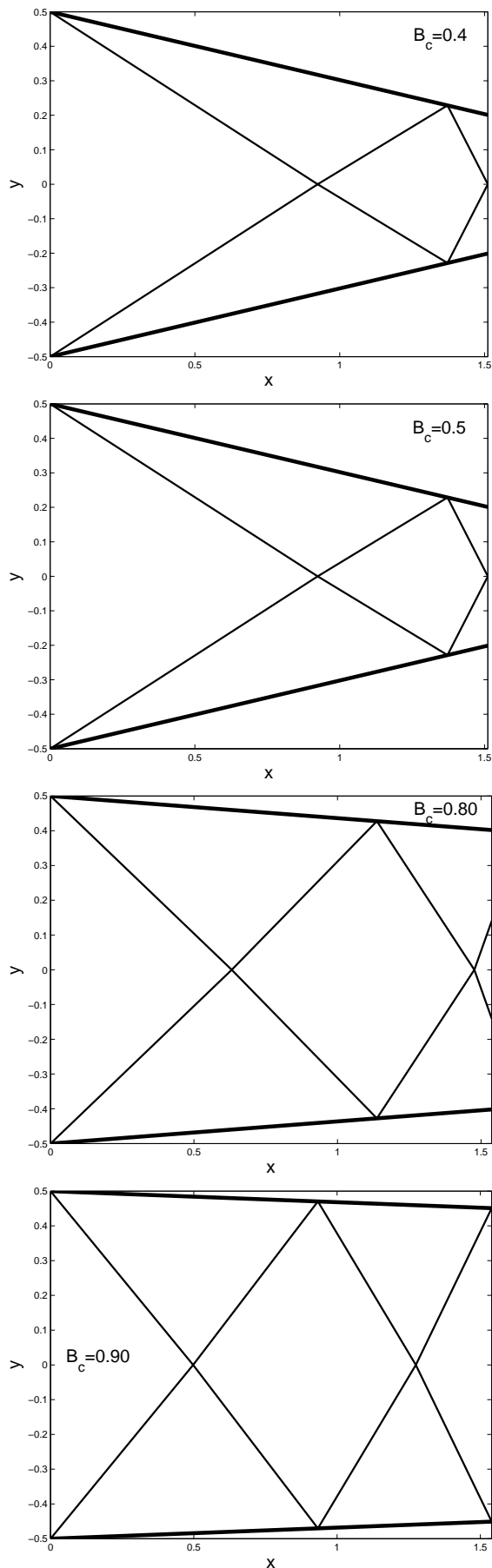
FIG. 11: Oblique jump patterns within the contraction for several values of B_c and minimal value of F_0 , and L = 0.3065\text{m} in scaled coordinates. The thick outer lines denote the contraction walls; the thin lines the oblique jumps.
