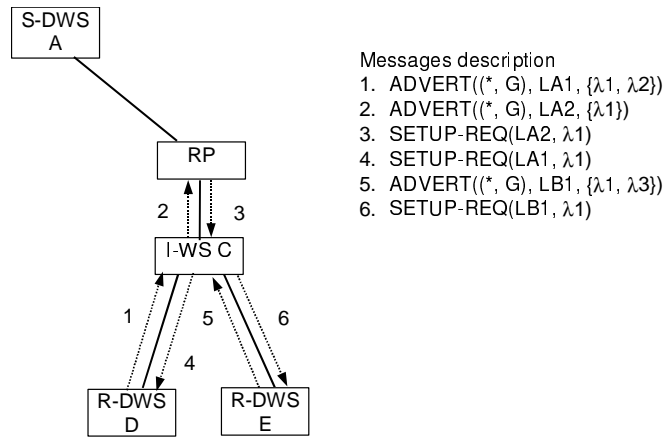
Figure 6 - RPT set-up example
