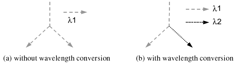
Figure 3 - Point-to-multipoint forwarding example
