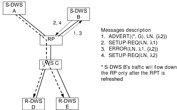
Figure 7 - Example of SPT set-up
