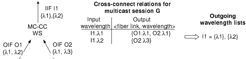
Figure 5 - Collecting mechanism example
