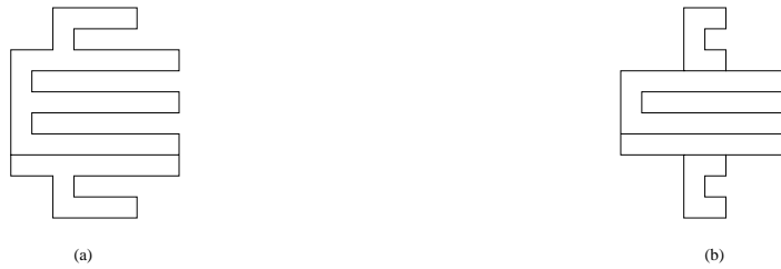
Figure 4: A Hamiltonian cycle for : (a) R(11, 10)^{-4(2,2)} (b) R(11, 10)^{-4(3,3)}
