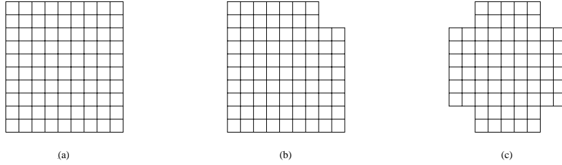
Figure 1: Truncated rectangular grid graphs : (a) R(11, 10) (b) R(11, 10)^{-1(2,2)} (c) R(11, 10)^{-4(2,2)}
