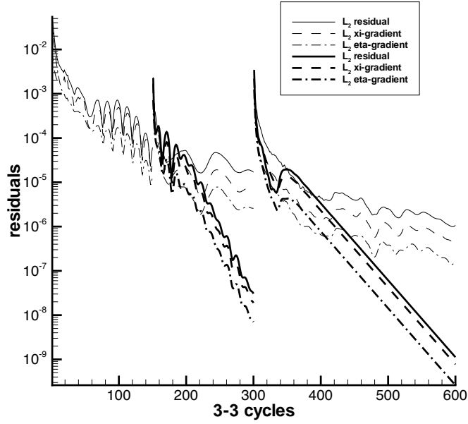
FIG. 4. Convergence rate comparison of the residual for the element mean and fluctuating DG coefficient equations using single and multigrid computations (dark lines) on a twice adapted mesh of a NACA 0012 airfoil.
