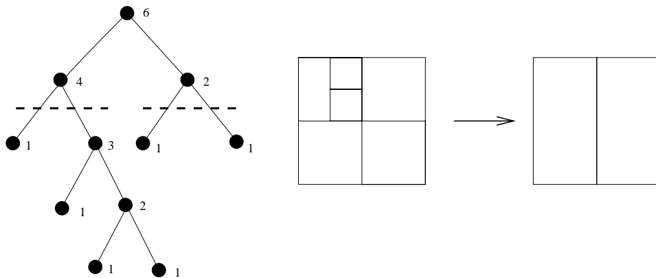
FIG. 2. Coarsening based on refinement tree. The numbers at the nodes of the tree refer to the number of leaves in the subtree. The dashed lines show where the tree is pruned. The fine grid cells and the resulting coarse grid cells are shown to the right.
