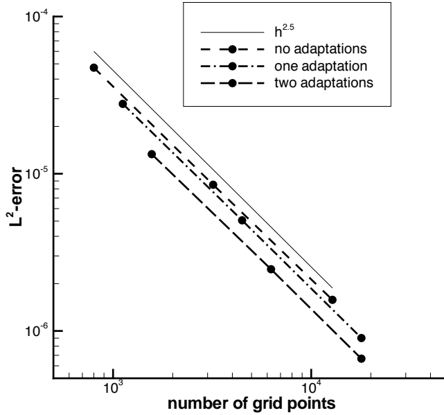
FIG. 10. L^2 -Error in flow calculations for converging-diverging channel on uniform and adapted meshes.
