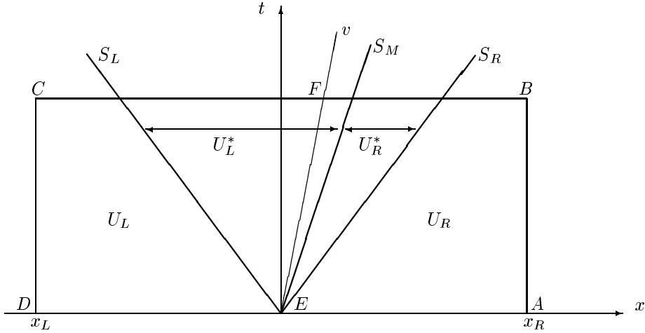
FIG. 1. Wave pattern used in the definition of the HLLC flux function for an element face moving with velocity v . Here S_L and S_R are the fastest left and right moving signal velocities. The solution in the star region U^* is divided by a wave with velocity S_M .
