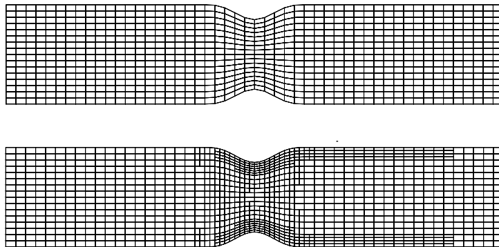
FIG. 9. Original and one time adapted mesh for converging-diverging channel.
