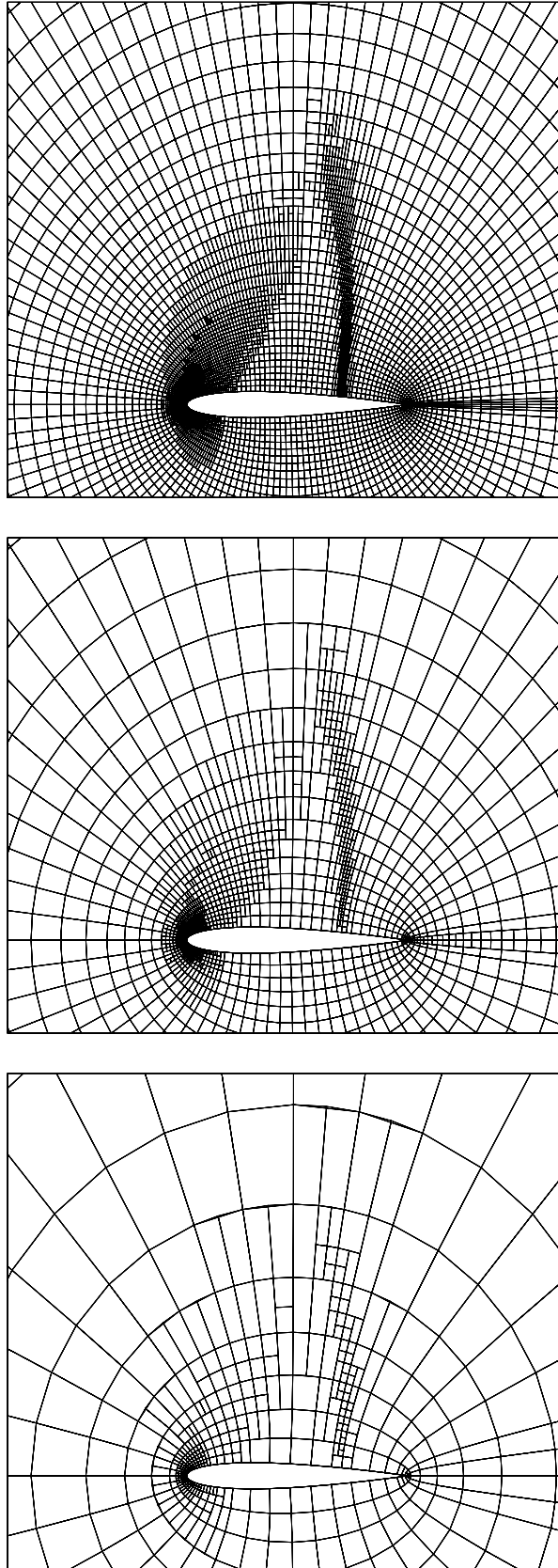
FIG. 3. Multigrid levels in an adapted mesh about the NACA 0012 airfoil.
