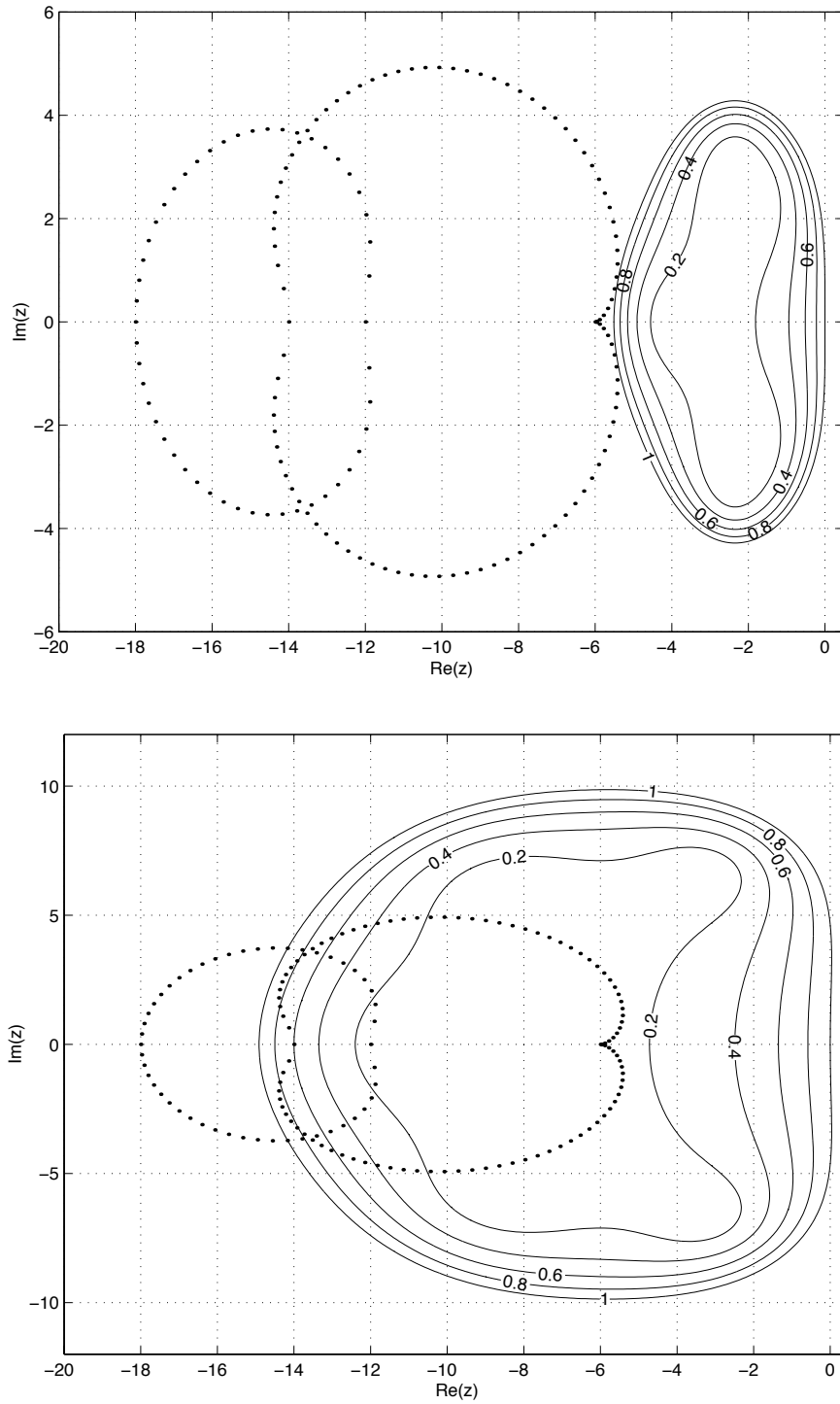
FIG. 6. Locus of the eigenvalues z_m(\theta) , \theta \in [0, 2\pi) , (dots) of the DG discretization of u_t + au_x = 0 and the stability domain of the explicit 5-stage Runge-Kutta method (40) with optimized coefficients (top) and the five stage semi-implicit Jameson Runge-Kutta scheme (bottom). CFL_{\Delta t} = 1.0 . CFL_{\Delta \tau} = 6.0 , no grid velocity.
