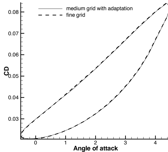
FIG. 11. Lift and drag coefficient on oscillating NACA 0012 airfoil ( M_\infty = 0.8 , \omega = \pi/10 ).
