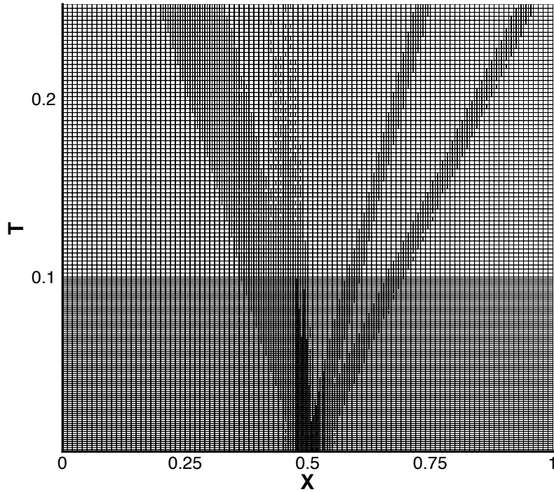
FIG. 7. Space-time mesh for the adaptive solution of Sod's shock tube problem.
