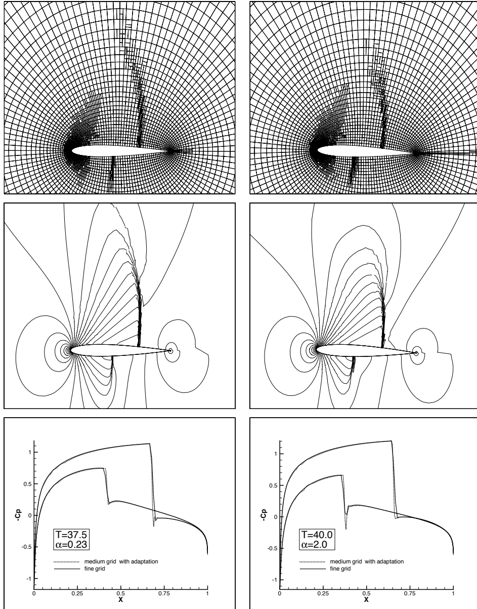
FIG. 13. Adapted mesh around oscillating NACA 0012 airfoil, contours of density, and pressure coefficient C_p on the airfoil surface for \alpha = 0.23^\circ (pitching upward) and \alpha = 2.0^\circ (pitching upward) ( M_\infty = 0.8 , \omega = \pi/10 ).
