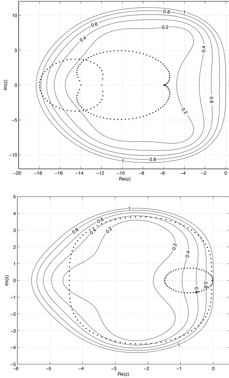
FIG. 5. Locus of the eigenvalues z_m(\theta) , \theta \in [0, 2\pi) , (dots) of the DG discretization of u_t + au_x = 0 and the stability domain of the 5-stage semi-implicit Runge-Kutta method with optimized coefficients. CFL_{\Delta t} = 1.0 , CFL_{\Delta \tau} = 6.0 (top), CFL_{\Delta t} = 100.0 , CFL_{\Delta \tau} = 2.2 (bottom), no grid velocity.
