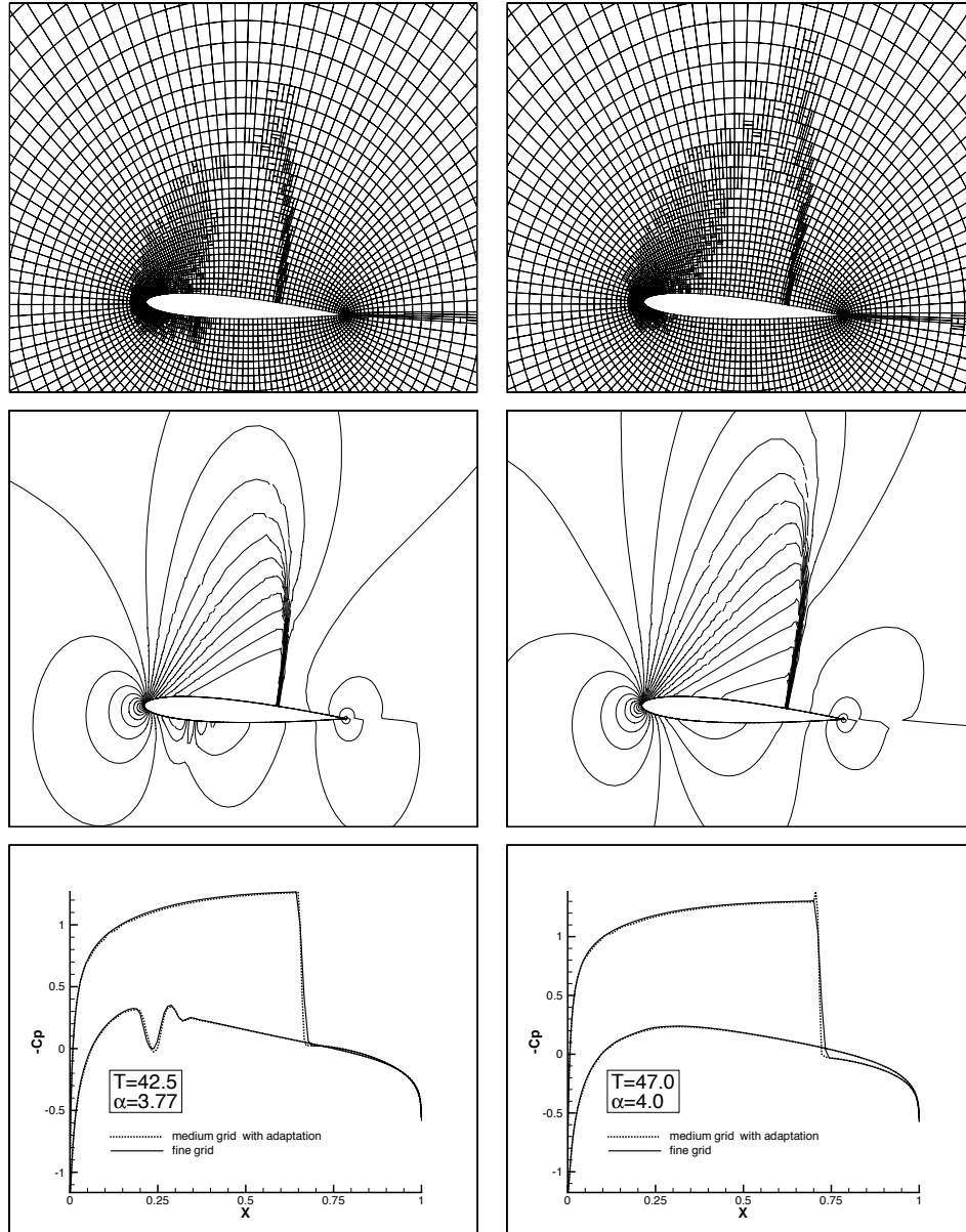
FIG. 14. Adapted mesh around oscillating NACA0012 airfoil, contours of density, and pressure coefficient C_p on the airfoil surface for \alpha = 3.77^\circ (pitching upward) and \alpha = 4.0^\circ (pitching downward) ( M_\infty = 0.8 , \omega = \pi/10 ).
