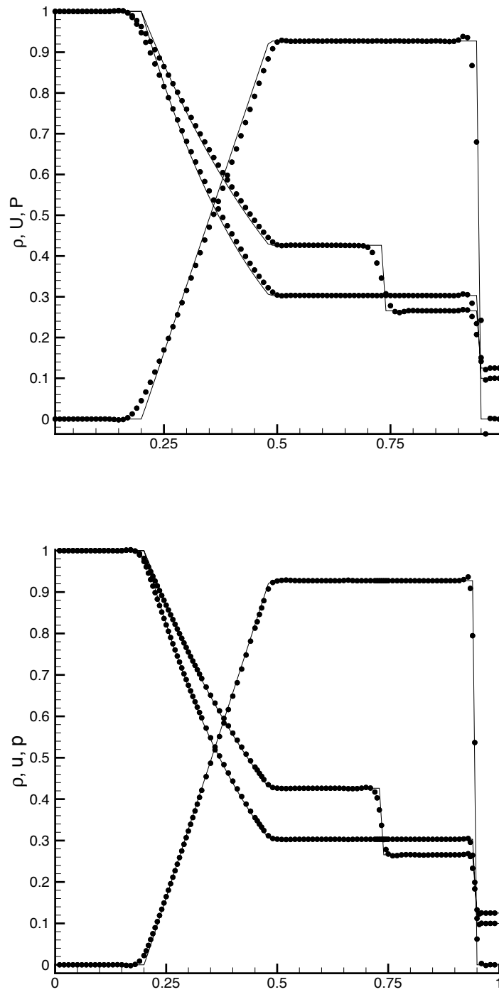
FIG. 8. Results of Sod's shock tube problem at t = 0.2531 on a uniform (top) and adapted mesh (bottom). Computed results plotted as circles, exact solution plotted as lines.
