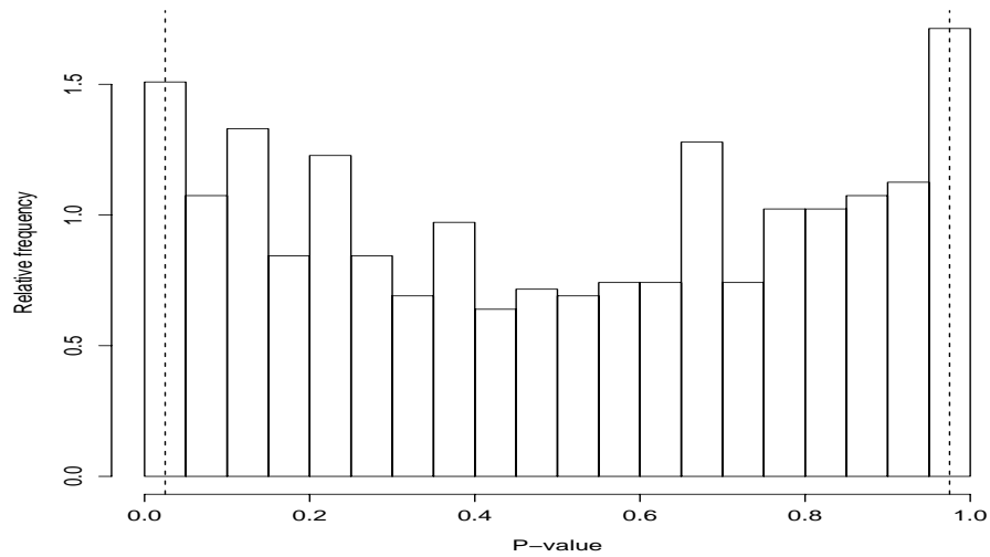
Figure 4. The p -values for the average item score statistic.
