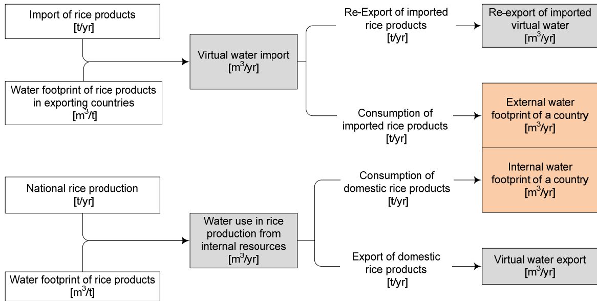
Figure 5. The calculation scheme for assessing the water footprint of national consumption of rice products.
