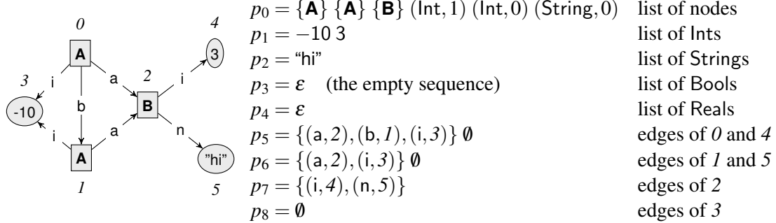
Figure 2: An example graph with |V| = 6 , represented by a state vector with |\vec{p}| = 9 . The canonical node numbers are in italics. Node labels A , B are self-edges; oval nodes are data values.
