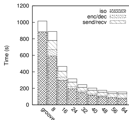
(b) Execution times for start-10.*
