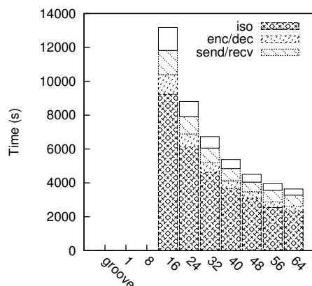
(c) Execution times for start-12.
