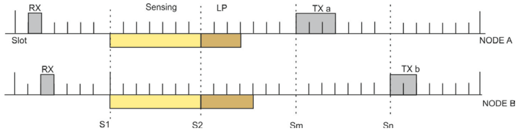
Figure 2. Schematic representation of wireless vibration monitoring with local processing
