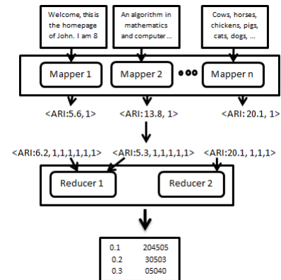
Figure 1: Visual overview of the MapReduce program
