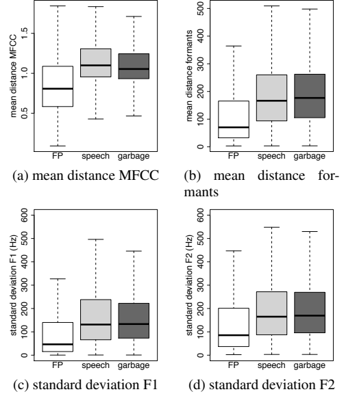
Figure 1: Box Whisker plots of various features for FP detection.
