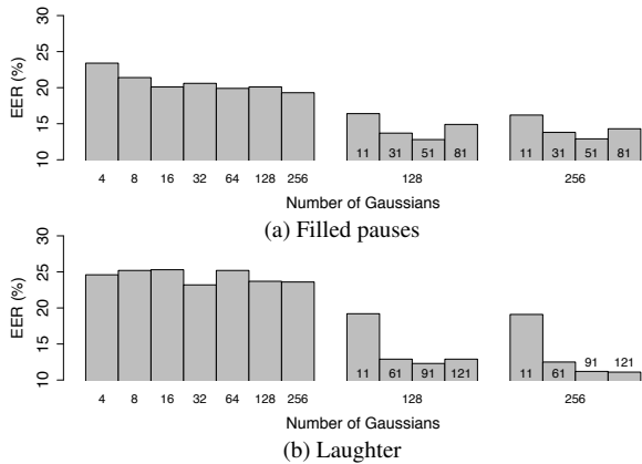
Figure 3: Results of GMMs trained with all features combined on feature-level. For N_{\text{gauss}} = 128 and 256 we show the EERs when median filters are applied.
