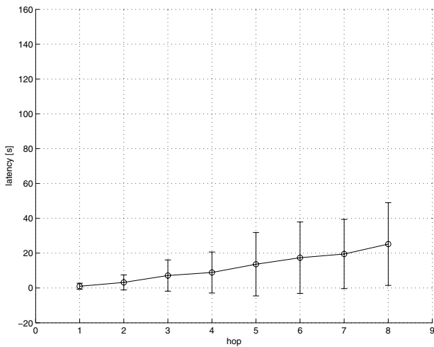
Fig. 5: Average latency and standard deviation; maximum given advice: 4 slots
