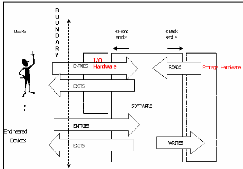
Figure 3. Generic flow of data attributes through software from a functional perspective [10]
