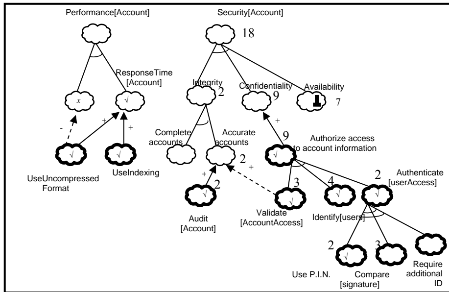
Figure 4: Calculating functional size for NFRs
