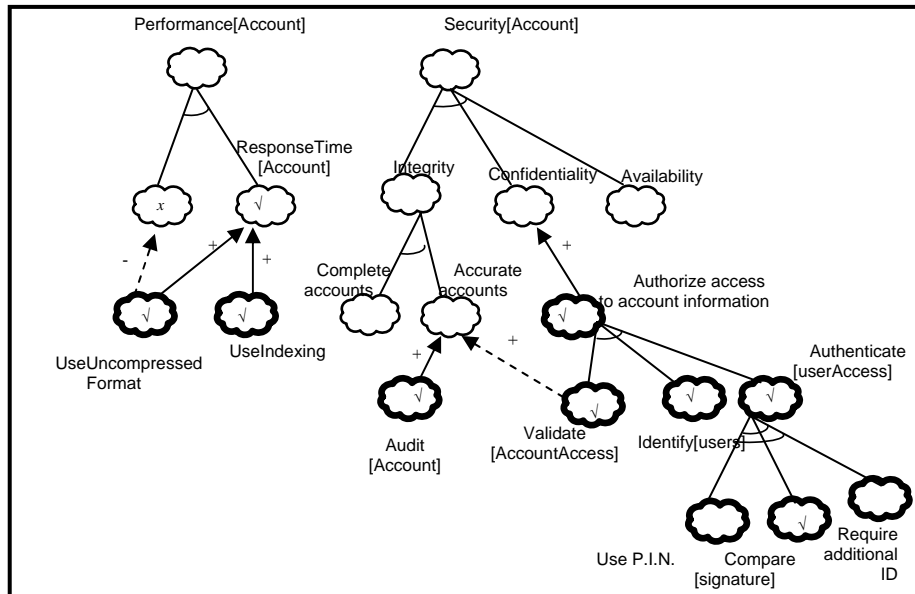
Figure 1. Softgoal interdependency graph for performance and security in a credit card system [4]
