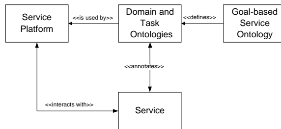
Fig. 1. Main components of our approach and their relationships.
