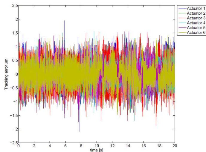
Figure 5: Measured tracking error of the actuator displacements during a 6 mm displacement of the end effector in the X,y -plane (from [13]).
