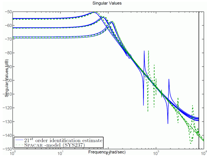
Figure 4: Singular values of the transfer matrix of the 21 th order identification estimate and the SPACAR-model near the equilibrium configuration (from [13]).
