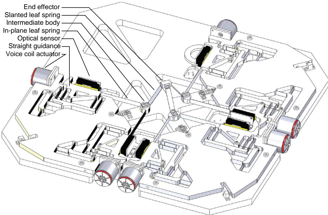
Figure 1: Six DOF hexapod-like manipulator with flexible joints [10].
