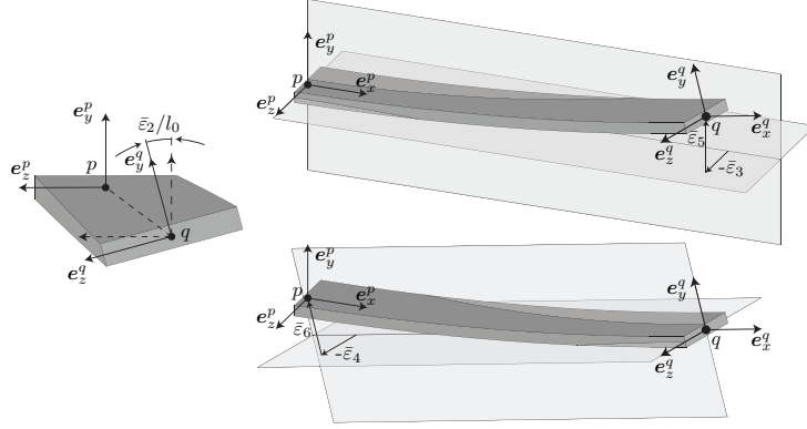
Figure 2: Deformations \varepsilon_2 - \varepsilon_6 of the spatial beam element (reprinted from [12]).
