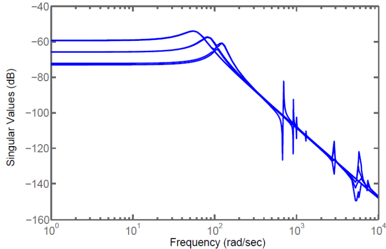
Figure 3: Singular values of the transfer matrix of the 237-DOF SPACAR-model near the equilibrium configuration (from [13]).
