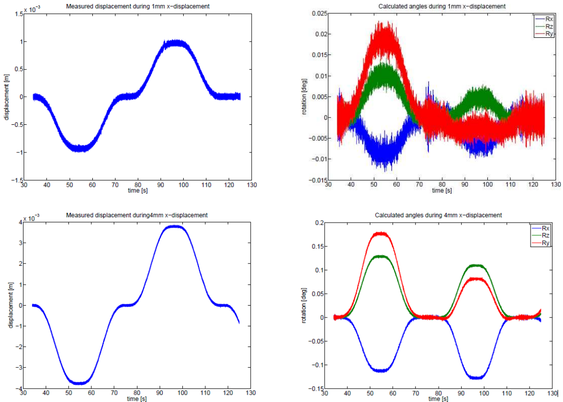
Figure 6: Measurements of the end effector motion during 1 mm (top) and 4 mm (bottom) x -displacements of the end effector. The left graphs show the long stroke motion in the x direction; the right graphs show all three rotations of the end effector for both displacements (from [13]).
