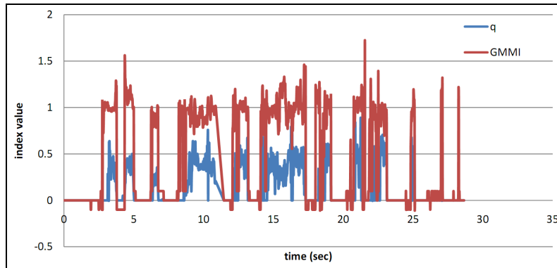
Fig. 5: Comparison between q_1 and GMMI mixing indices for a single cell at the bottom of the mixer. The zero values correspond to the times when the cell is empty.
