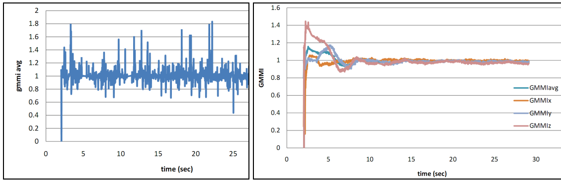
Fig. 4: (Left) Average GMMI value of all cells with the reference point at the bottom of the mixer. (Right) Average GMMI and directed GMMIs of all cells with the reference point at the centre of each cell.
