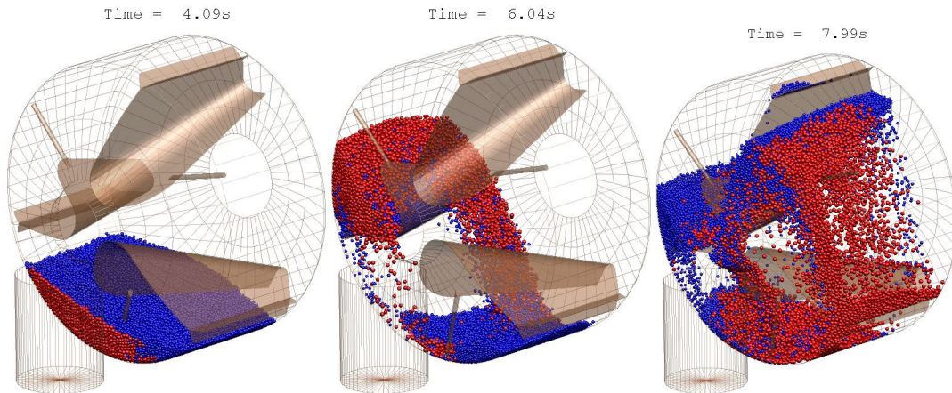
Fig. 2: Picture sequence from a DEM simulation with 10 rpm, rotation is clockwise, of a binary distributed particle system in a Lindor mixer (left) after filling, just before rotation starts, (middle) after the first blade has moved 1/3, i.e., half-way up, and (right) after the first blade has moved 2/3 around.
