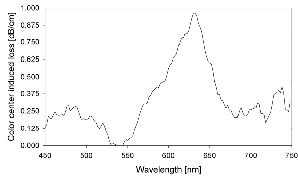
Fig. 2. Color-center induced loss spectrum of a fs-laser written waveguide
