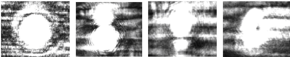
Fig. 1. Near-field mode profiles of fs-laser written waveguides. a) fundamental mode b) 1 st order mode, c) 2 nd order mode, d) ‘donut’ mode
