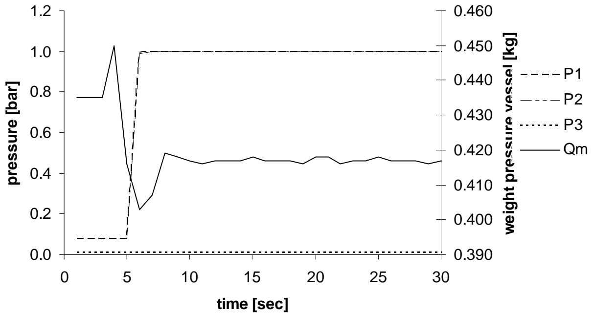
Fig 7 Pressure and flow rate versus time preform under compression to 55% V_f
