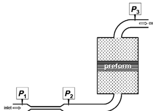
Fig 4 Location of the pressure transducers
