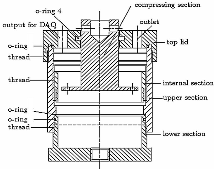
Fig 1 Composition drawing of the design of the permeability instrument.
