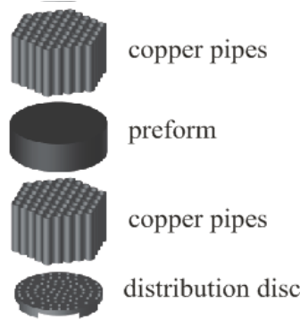
Fig 2 The position of the copper pipes in relation to the preform.
