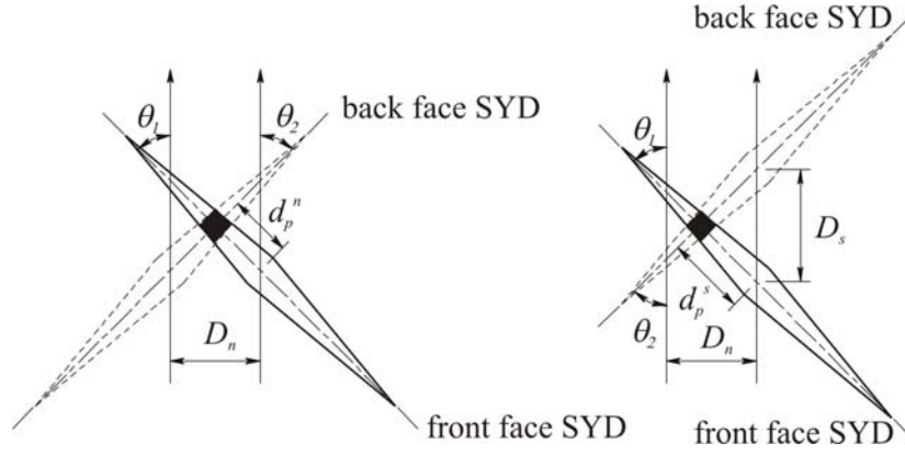
Fig. 2 Locations of overlap regions (dark areas) depend on integer multiplications of the projected distance d_p^n and d_p^s on the SYD. \theta_1 is the fibre angle of the upper layer, \theta_2 the fibre angle of the bottom layer.
