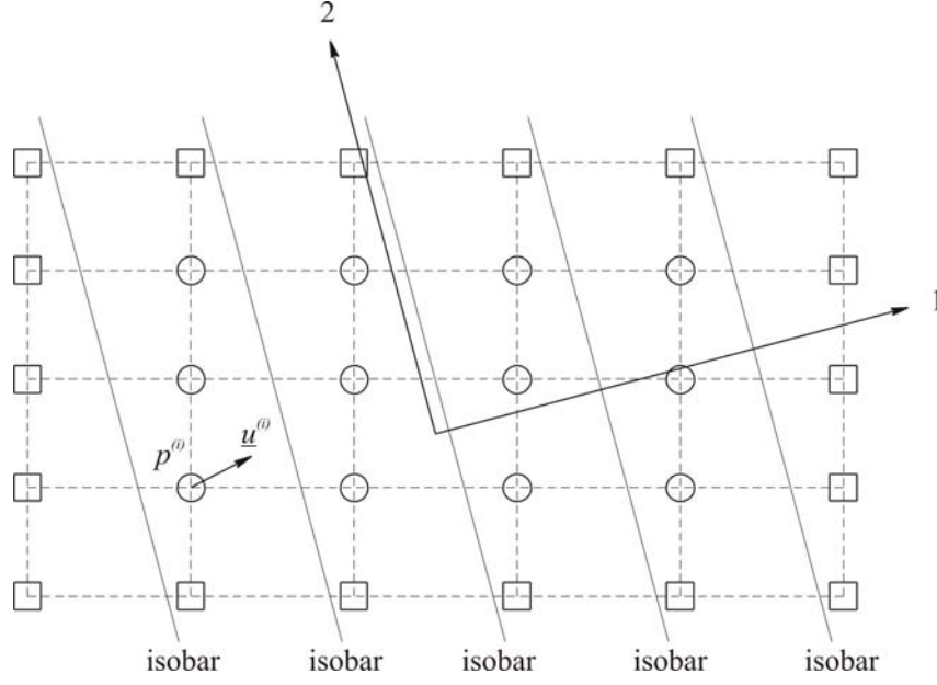
Fig. 5. Grid of interaction points (circles: inner points, squares: outer points at which the boundary conditions are applied). 1 and 2 refer to the principal directions, the pressure p and fluid velocity \underline{u} at point i are indicated. Isobars visualise the assumed linear pressure gradient.
