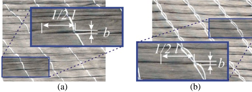
Fig. 1. Stitch Yarn induced fibre Distortions on the top and the bottom face of a \pm 45^\circ biaxial Non-Crimp Fabric, with a chain knit pattern. b is the width and l the length of the SYD.
