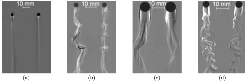
Figure 6. Stereoscopic views of rising spheres and their wake structures observed at several Reynolds numbers (Reynolds number increases from a to d and continues in figure 7). The left part of each frame shows the xz -plane and the right part the yz -plane. Values of the parameters d , \rho_s/\langle\rho\rangle , G and Re_T are, respectively: (a) 3.2 mm, 0.97, 121, 210; (b) 4.0 mm, 0.88, 334, 565; (c) 8.0 mm, 0.99, 331, 602; (d) 6.4 mm, 0.93, 534, 920.
