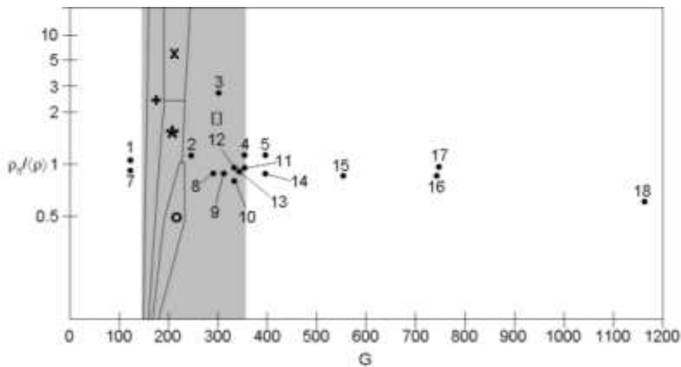
Figure 5. Phase diagram: density ratio \rho_s/\langle\rho\rangle versus Galileo number. The grey box is the regime analysed by Jenny et al. [8]. They find in the most left region an axisymmetric wake. The symbols, directly taken from [8], denote: + steady and oblique, * oblique and oscillating regime with low frequency ( 0.045 \leq f \leq 0.068 ), \times oblique and oscillating regime with high frequencies ( f = 0.180 ), O zigzagging periodic regime ( 0.023 \leq f \leq 0.035 ) and \square chaotic regime. The numbers denote the number of our experiment in table 1. Experiments 6 and 19 fall outside the diagram.
