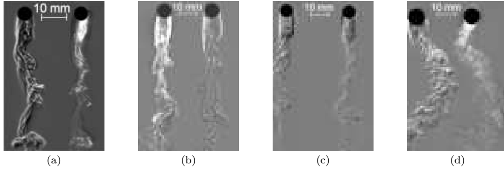
Figure 7. Stereoscopic views of rising spheres and their wake structures observed at several Reynolds numbers (Reynolds number increases from a to d). The left part of each frame shows the xz -plane and the right part the yz -plane. Values of the parameters d , \rho_s/\langle\rho\rangle , G and Re_T are, respectively: (a) 6.4mm, 0.87, 728, 1180; (b) 7.9 mm, 0.93, 732, 1350; (c) 6.4 mm, 0.65, 1160, 1965; (d) 9.5 mm, 0.50, 2548, 4623.
