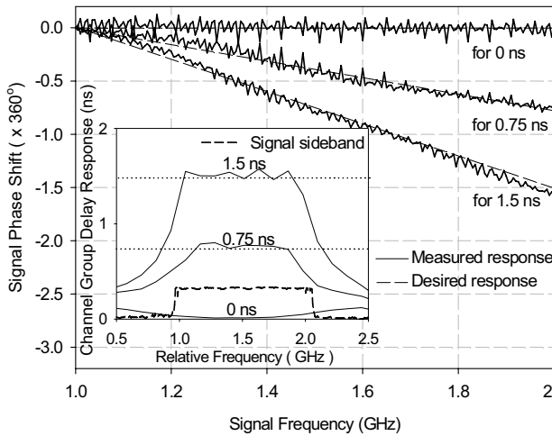
Fig. 4: Signal phase shift for different channel delays
