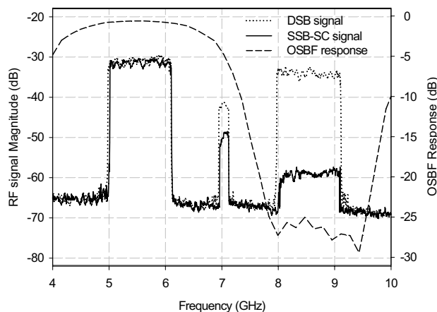
Fig. 3: Filter-based optical SSB-SC modulation
