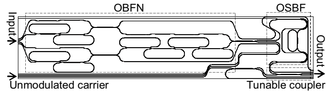
Fig. 2: Waveguide layout of an integrated beamformer chip
