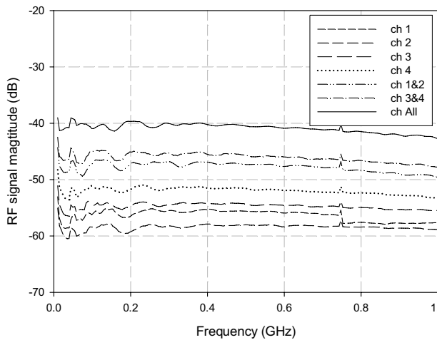
Fig. 5: RF magnitude responses for individual channels and signal combination.
