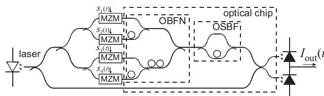
Fig. 1: Schematic of the beamformer system
