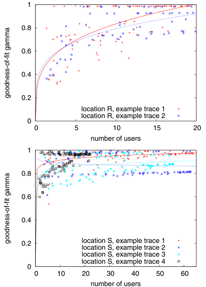
Fig. 8. Gaussianity compared to number of active users
