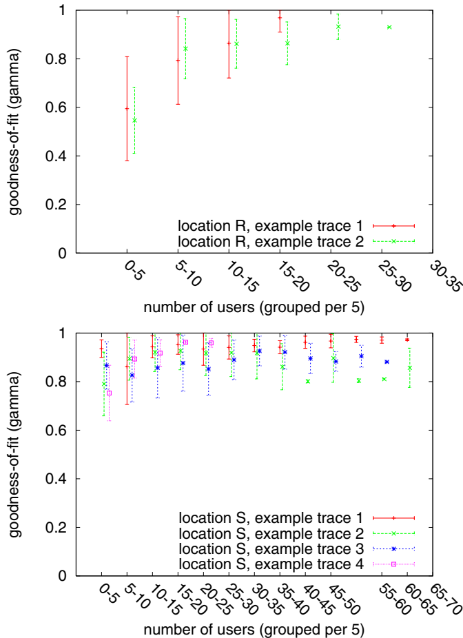
Fig. 7. Gaussianity compared to number of active users (grouped)
