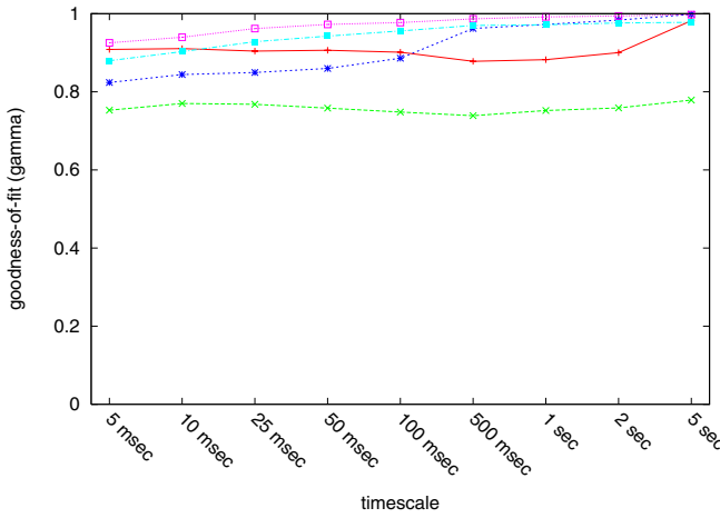
Fig. 4. Comparing Gaussianity at different timescales, for 5 example traces from location R.
