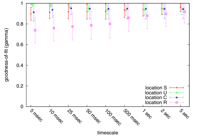
Fig. 6. ‘Average Gaussianity’ at different timescales for all locations
