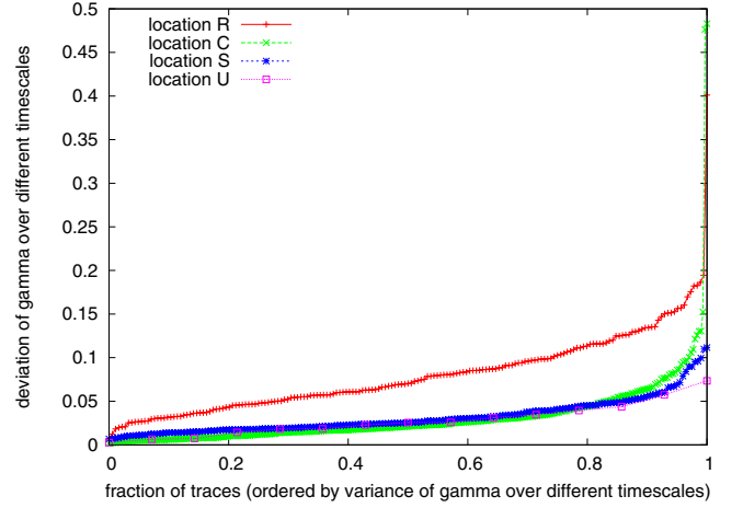
Fig. 5. \nu_\gamma : goodness-of-fit \gamma over different timescales
